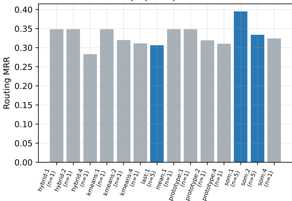
gasper, split 32
