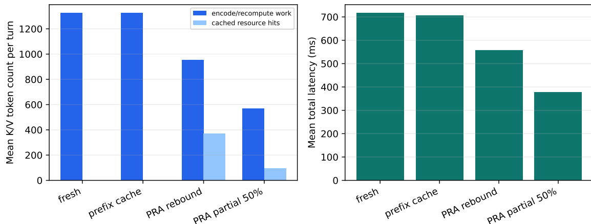
Figure 13: Five-seed mean per-turn K/V accounting and measured latency under changing selections. Encoding/recomputation and cache hits are shown as separate bars rather than as an active-context stack. Diagnostic repair is omitted because copying precomputed fresh states is not a deployable timing.
