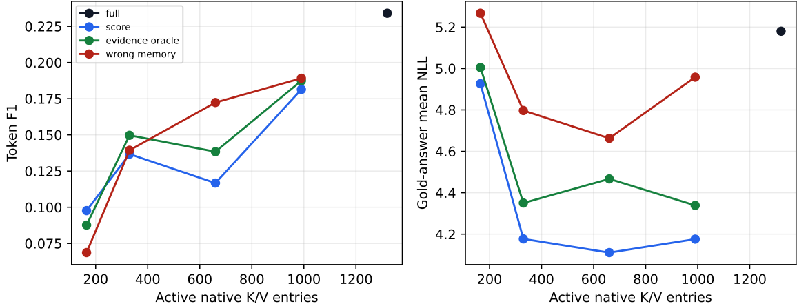
Figure 12: Quality and gold-answer NLL against active native K/V. The different metrics need not rank small-sample generations identically.
