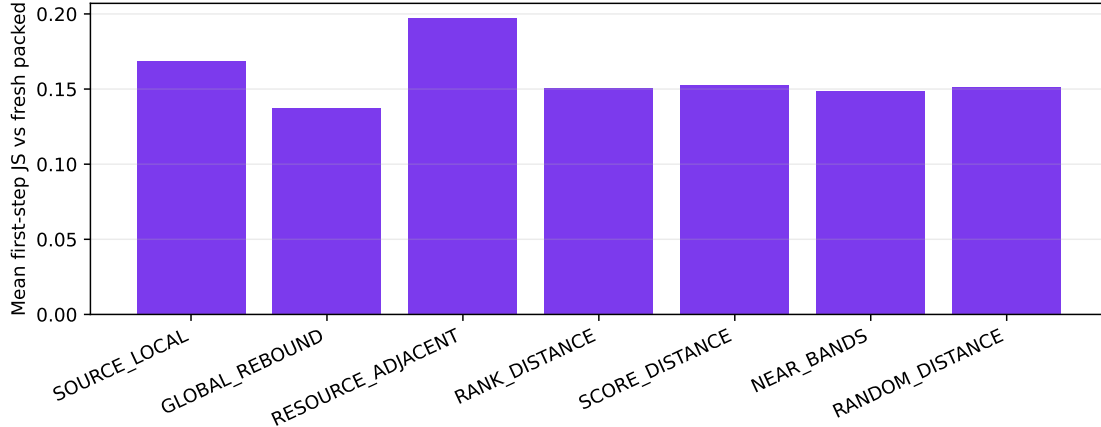
Figure 11: First-step divergence from fresh packed encoding under alternative position policies (200 order-specific comparisons per policy across five cohorts).
