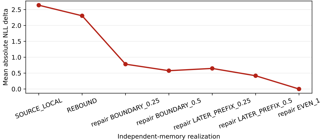
Figure 10: Position rebinding and deterministic contextual repair reduce the composition error, but all five cohorts reach exact parity only at full repair. Repair timings are diagnostic because fresh packed states were computed first.
