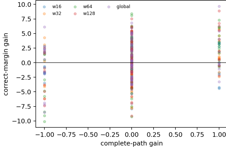
Figure 9: Paired complete-path and correct-margin changes. Positive path changes usually move the frozen decision in the correct direction, but most rows do not improve the path.
