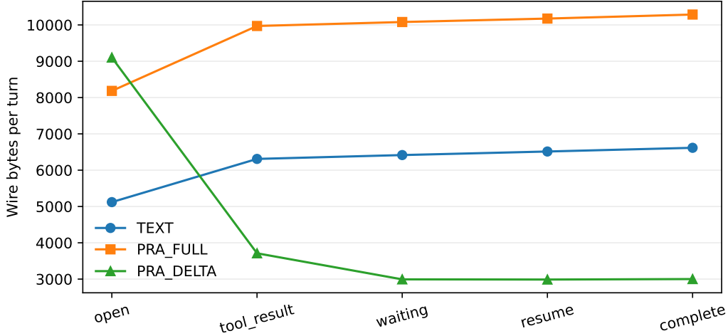
Figure 14: Per-turn JSON bytes for the five-turn task/tool workflow. PRA-FULL preserves explicit metadata but repeats all resource bodies; PRA-DELTA sends a body only for ADD or UPDATE and keeps unchanged resources logical.
