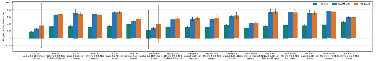
Figure 23: HOT, WARM, and COLD request p50 with p95–p50 upper whiskers. WARM recovery is reliable, but synchronous promotion remains visibly expensive.
