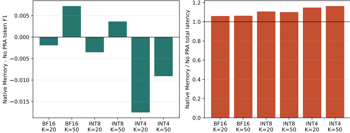
Figure 32: Quality and latency changes for the matched BF16, INT8, and INT4 deployed pipelines. The small one-seed cohort is directional evidence, not a precision invariance claim.
