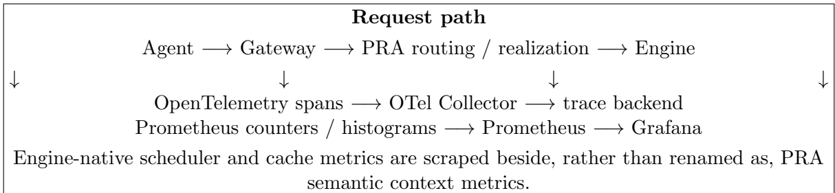
Figure 36: The observability boundary. W3C context joins request causality, while Prometheus and Grafana correlate semantic context decisions with engine-native serving behavior.
