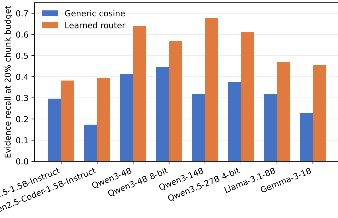
QASPER
