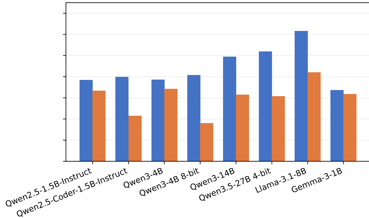
HotpotQA
