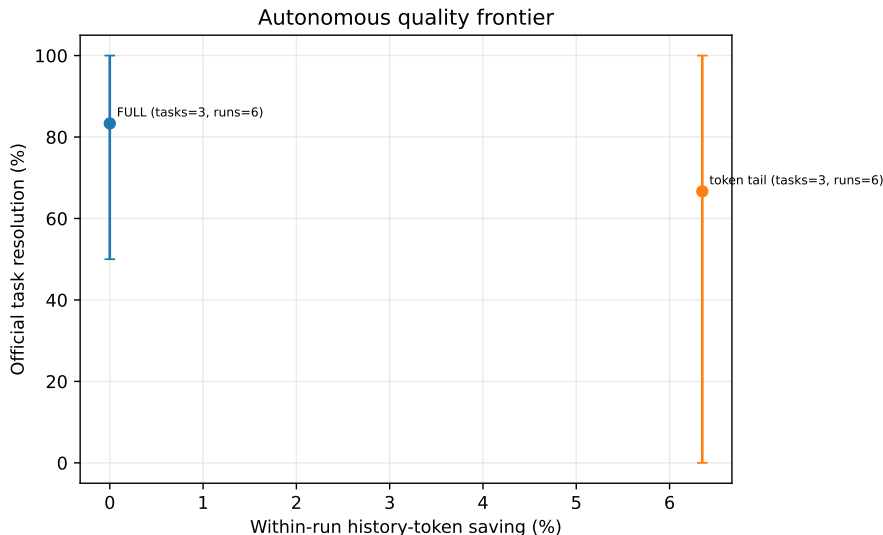
Figure 2: The first autonomous accuracy-saving point. Error bars are task-clustered and necessarily wide for three identities. The tail policy is not promoted because its point lies below the predeclared quality gate.
