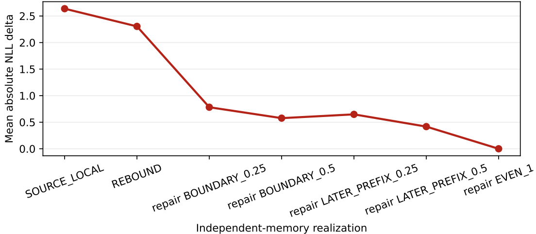
Figure 8: Position rebinding and deterministic contextual repair reduce the composition error, but all five cohorts reach exact parity only at full repair. Repair timings are diagnostic because fresh packed states were computed first.
