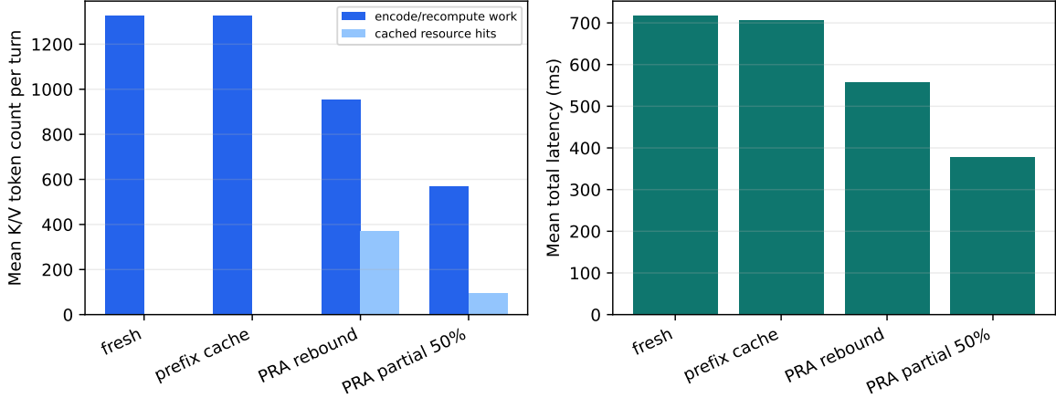
Figure 11: Five-seed mean per-turn K/V accounting and measured latency under changing selections. Encoding/recomputation and cache hits are shown as separate bars rather than as an active-context stack. Diagnostic repair is omitted because copying precomputed fresh states is not a deployable timing.
