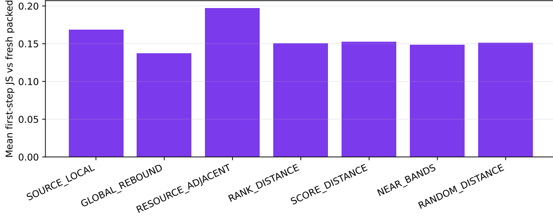
Figure 9: First-step divergence from fresh packed encoding under alternative position policies (200 order-specific comparisons per policy across five cohorts).
