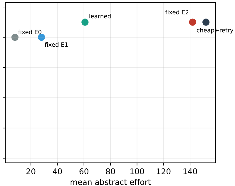
qasper
