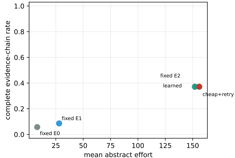
hotpotqa
