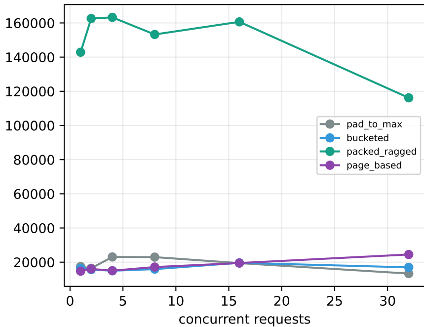
prototype throughput (requests/s)
