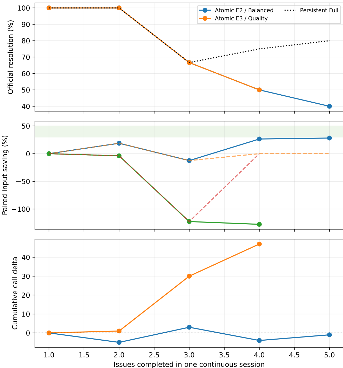
Easy-14 atomic instruction-epoch frontier (descriptive)
