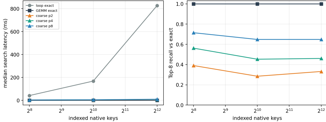
Figure 7: Native-Q/K search. Exact GEMM removes Python per-key overhead. The present deterministic coarse index loses recall and does not yet beat GEMM at these memory sizes.
