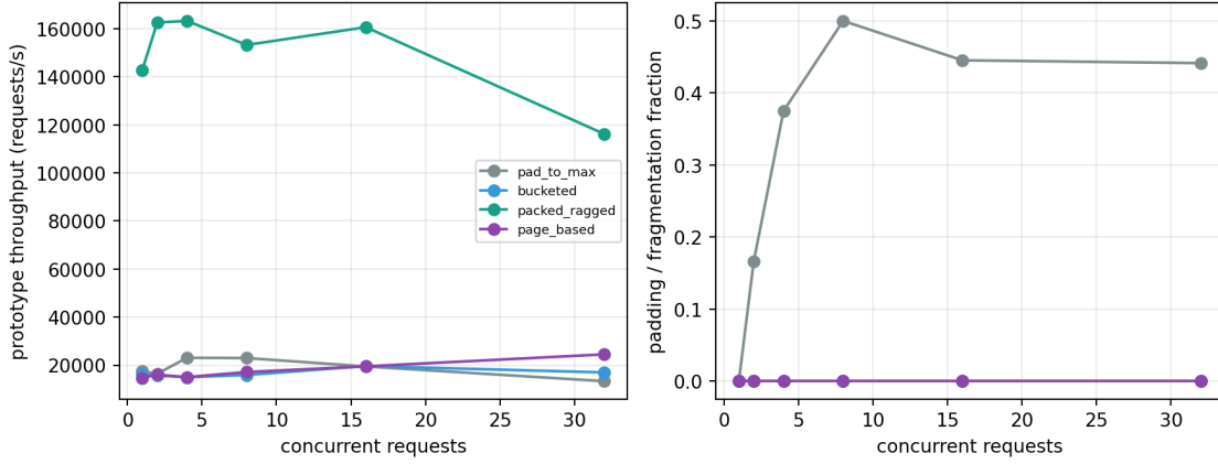
Figure 8: Controlled CPU batching. Packed ragged execution avoids padding and is fastest for this small per-request matrix-vector workload; this is not a GPU attention-kernel benchmark.
