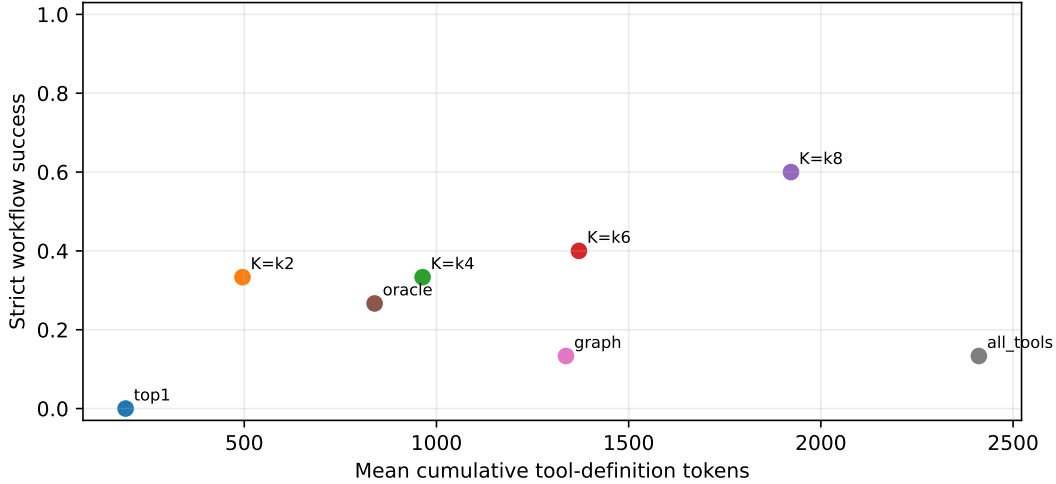
Figure 17: E4 strict workflow success against cumulative visible schema tokens. The frozen model, host authorization, and pure handlers are unchanged across candidate policies.
