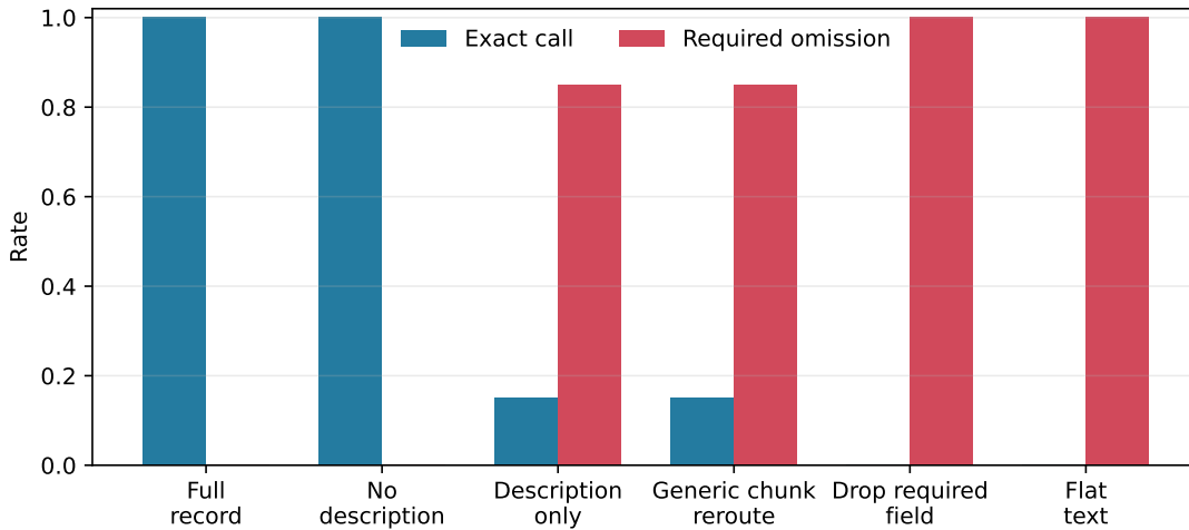
Figure 18: E5–E6 exact calls and required-argument omissions. The generic router selects one internal schema segment; all partial-schema conditions are experimental controls, not runtime fallback policies.
