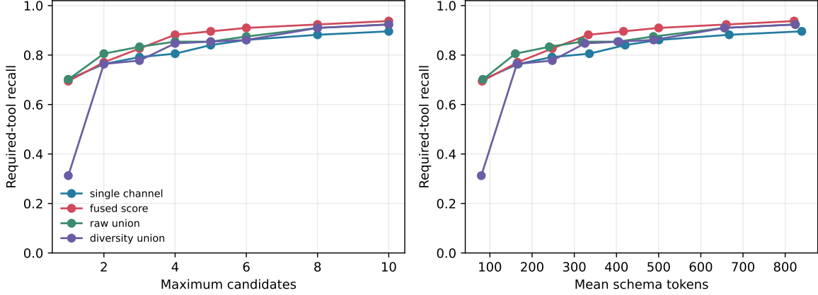
Figure 16: E2 required-tool recall against candidate count and serialized schema cost. Diversity preserves channel representation but does not dominate fused Top-K at matched budgets.
