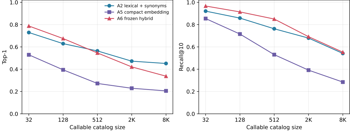
Figure 25: Top-1 and Recall@10 under five seeded callable catalogs. The A6 mixture is frozen rather than retuned at each scale.
