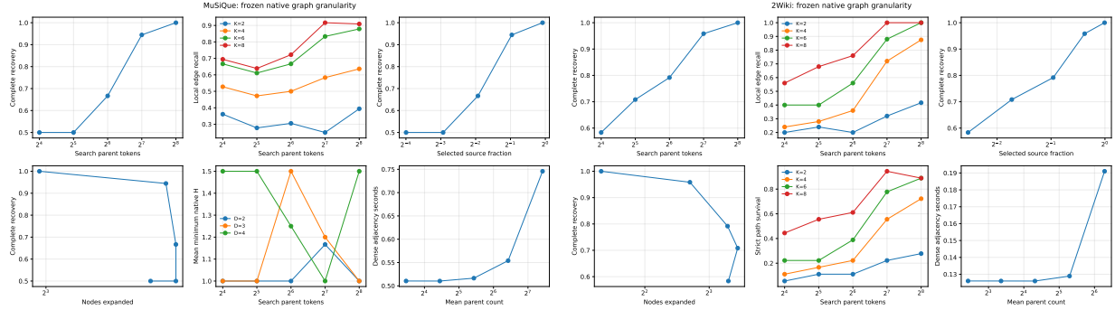
Figure 13: Granularity changes both conceptual payload and complete evidence recovery. Fine memory is sparse but topologically fragile; coarse memory is reachable but distractor rich.
