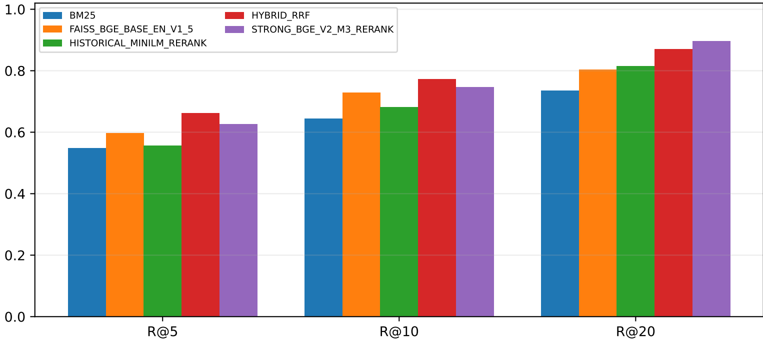
Supporting-document recall
