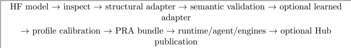
Figure 29: The model-onboarding path. Each arrow is a separately inspectable service boundary rather than an implicit side effect of one CLI callback.
