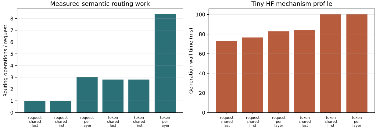
Figure 2: Five-seed tiny-HF mechanism profile. Routing operations validate the execution contract; wall time is host- and model-specific and is not a serving speed claim.
