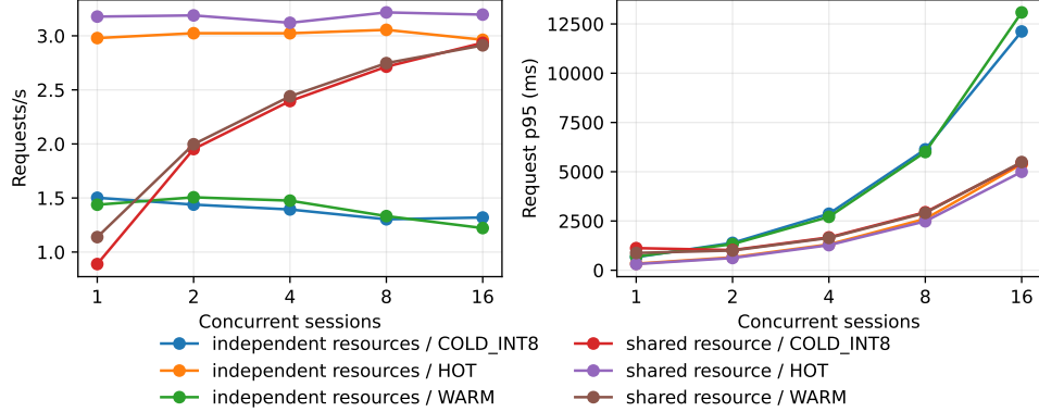
Figure 20: Shared and independent MLX resources through 16 concurrent sessions. The finite waves include promotion and serialized model queueing.
