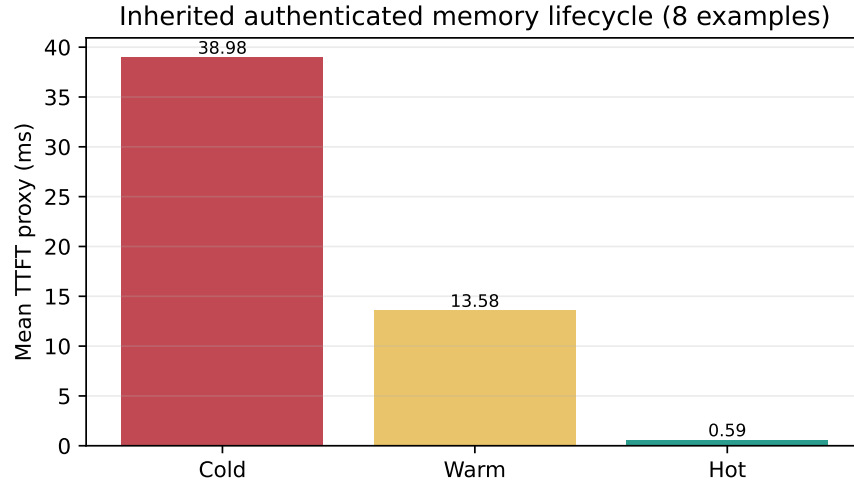
Figure 11: Inherited Paper 4 lifecycle proxy over eight examples. Cold includes fetch and native encoding; warm reuses native encoding; hot reuses selected K/V.
