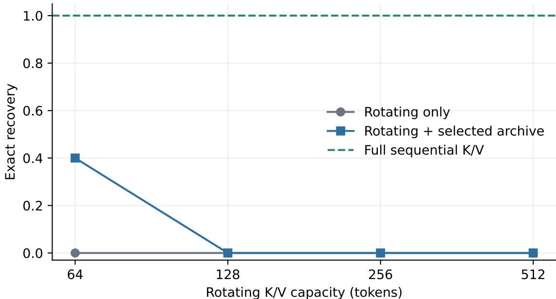
MLX rotating-cache archive control (5 seeds)
