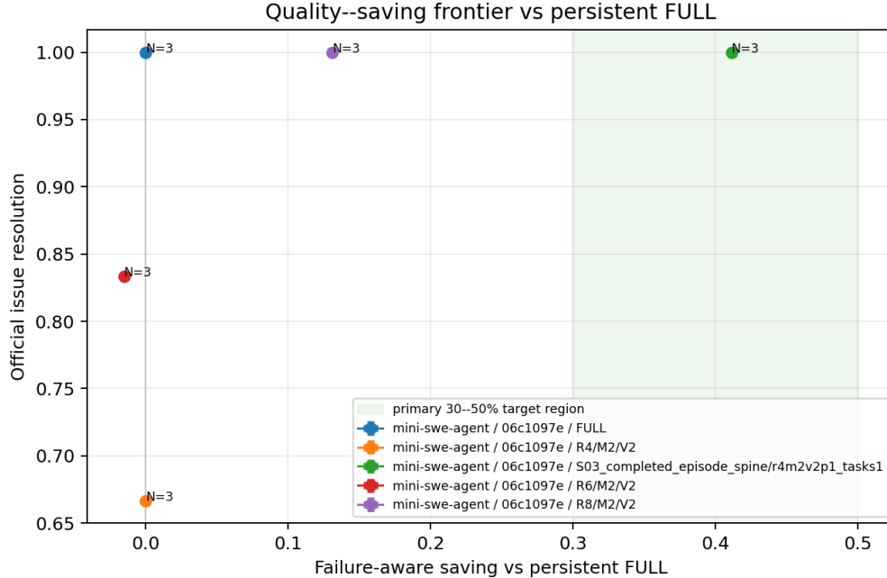
Figure 2: Failure-aware quality–saving frontier for the replacement N=3 cohort. The shaded band is the predeclared 30–50% target; P1 enters it while preserving all paired successes in both executions. Error bars are absent because this cohort contains only one ordered sequence family.
