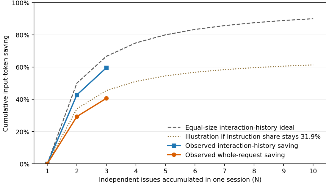
Figure 2: Empirical fixed-trajectory opportunity at N=1-3 and analytic equal-size scaling to N=10 . The dotted whole-request line holds the observed N=3 instruction share fixed only to illustrate the denominator effect; it is not a forecast because the immutable prompt share can change with N .
