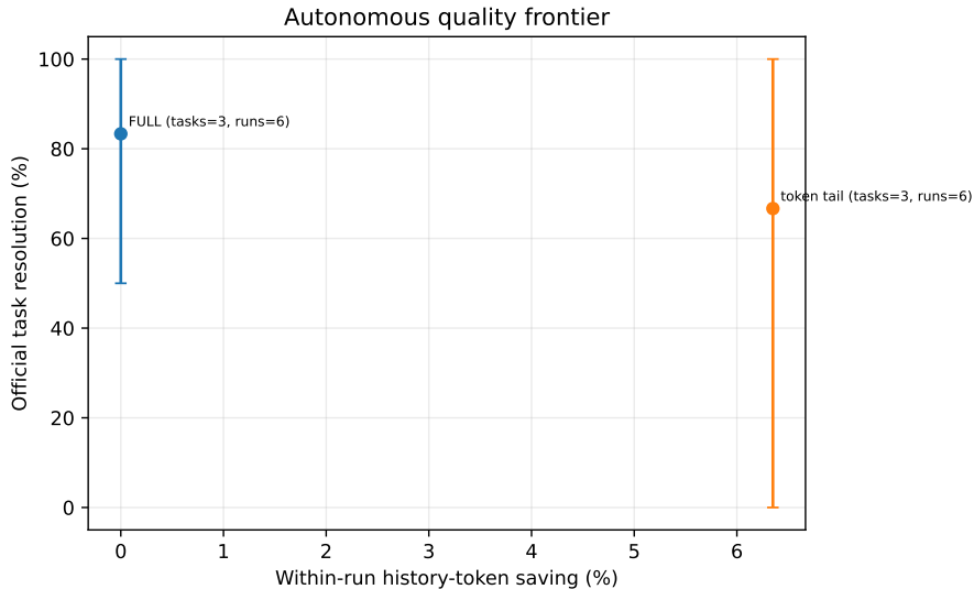
Figure 4: The first autonomous accuracy–saving point. Error bars are task-clustered and necessarily wide for three identities. The tail policy is not promoted because its point lies below the predeclared quality gate.
