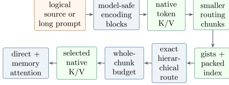
Figure 1: End-to-end PRA pipeline. Large logical sources are contextualized in bounded encoding blocks, then sliced into smaller addressable routing chunks. Gists select chunks; the budgeter admits complete native token K/V; and selected memory joins direct context in ordinary attention.
