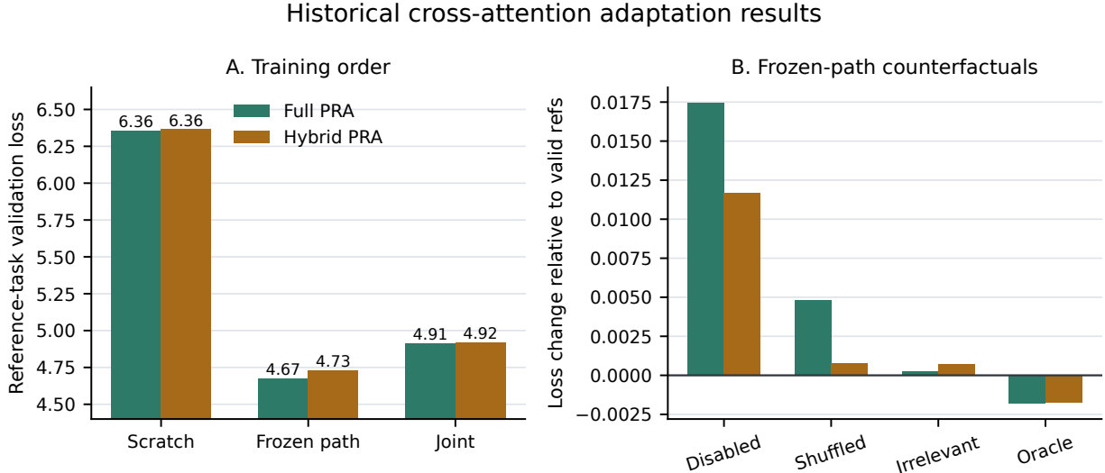
Figure 26: Historical cross-attention adaptation results. Left: frozen-path adaptation finishes substantially below scratch and direct joint tuning for both PRA placements. Right: frozen-path loss changes relative to valid references; positive values are worse. Disabling memory has a visible cost, but shuffled and irrelevant changes and oracle gains are small, so the branch effect is not evidence of content-causal retrieval.
