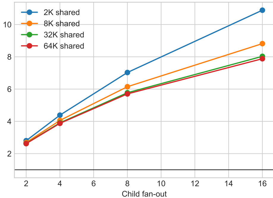
Injected-cost break-even surface
