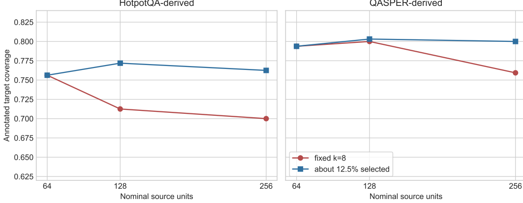
Figure 2: Fixed breadth becomes increasingly sparse as candidate count grows. Holding the selection fraction near 12.5% yields stable annotated target coverage through 256 units.
