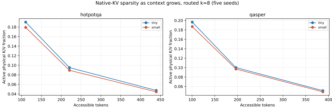
Figure 3: Fixed k = 8 keeps the selected physical payload nearly constant as candidate count grows, causing the active fraction to fall.
