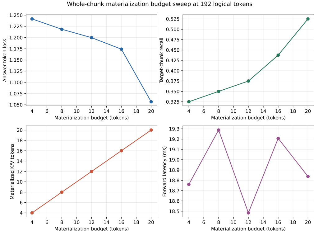
Figure 4: Quality and target recall improve as more of the 32-token operation budget is assigned to materialized memory.
