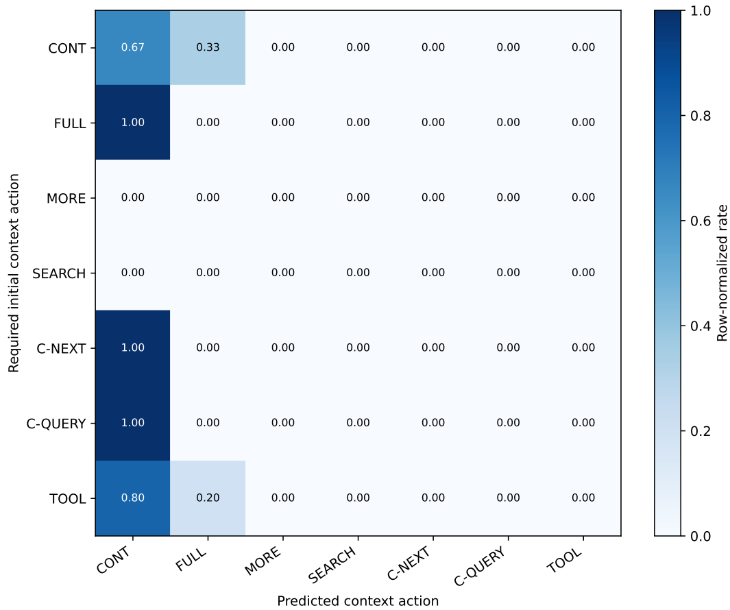
Figure 8: Row-normalized PRA-plus-model context-action confusion. Targets are evaluated after PRA automatic selection; C2 and C4 become CONTINUE when PRA has already exposed their evidence.
