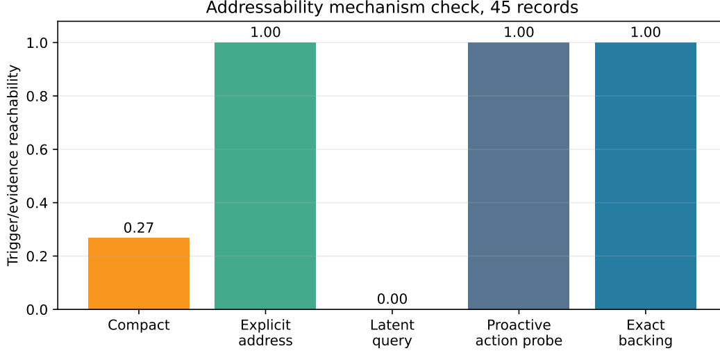
Figure 13: Compact visibility and addressability are different properties. Explicit and candidate-action probes use retrieval-only views; exact backing is hash-verified full recovery.
