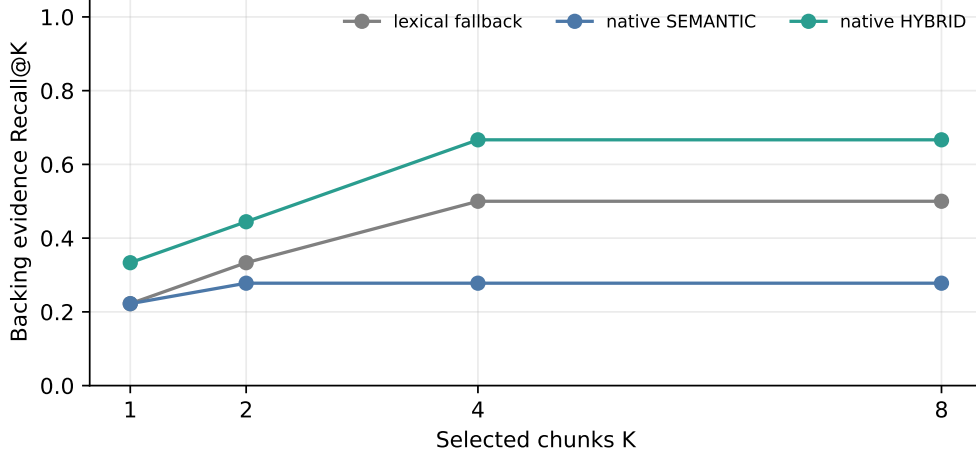
Figure 2: Pure full-backing evidence reachability. Lexical fallback is retained as a transparent mechanism control; semantic and hybrid curves use production hidden-state routing and original native-K/V spans.
