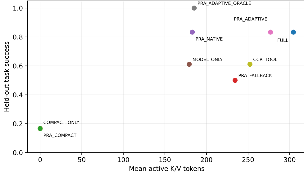
Figure 5: Held-out task success versus active K/V. Ingestion and address-index storage are reported separately and are not charged as active prompt/KV context.
