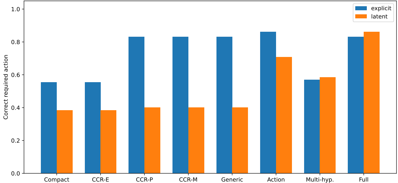
Figure 14: Final required-action accuracy for explicit and latent queries. Full context is a model ceiling rather than a deployable recovery policy. Action-conditioned search improves latent discovery but expands multiple candidate records.
