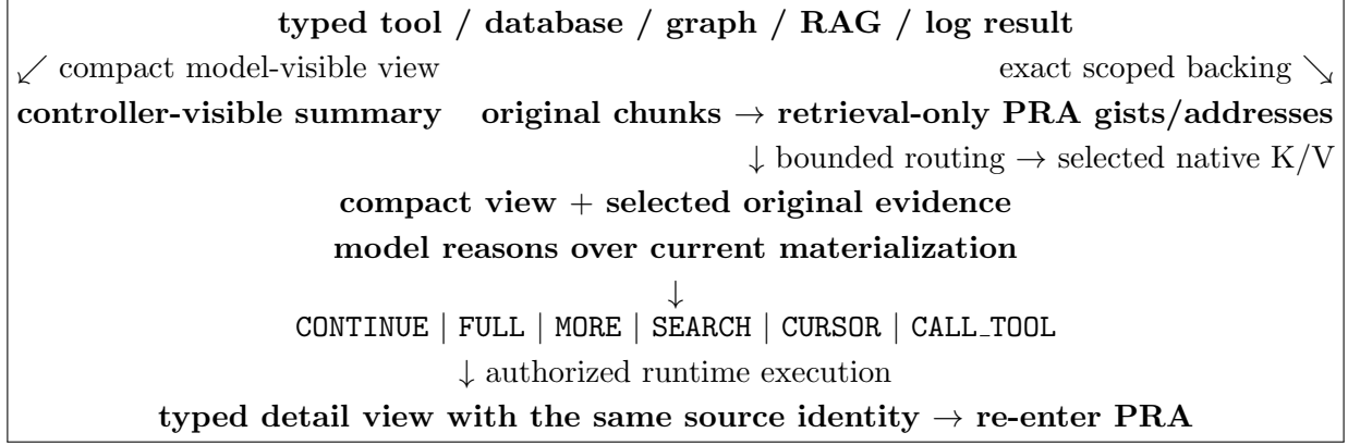
Figure 1: The corrected Paper 7 control loop. Visible compression and PRA address encoding are separate. Production PRA performs discovery over exact backing chunks before the model performs escalation selection. Every expansion is an authorized typed view and recursively re-enters PRA.
