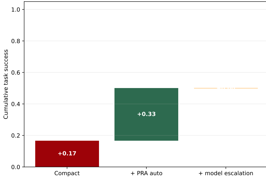
Figure 11: Task-success decomposition. The measured gain over compact-only is provided by PRA automatic selection; this frozen controller adds no net task success after PRA.
