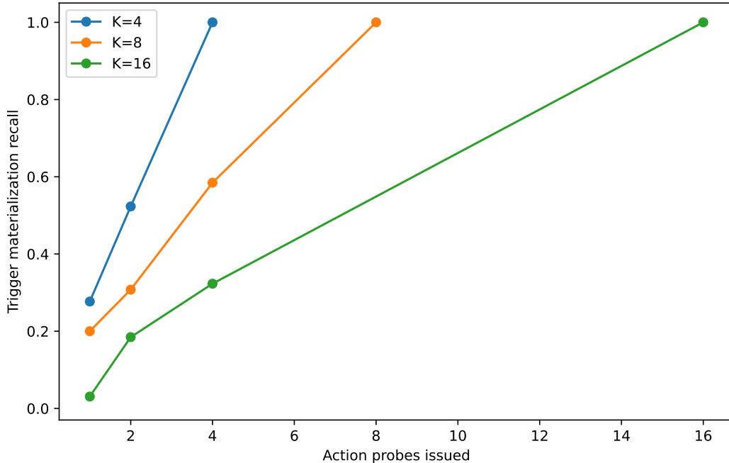
Figure 16: Trigger materialization against probes issued for palettes of K \in \{4, 8, 16\} . Exhaustive action probing is an interpretable upper bound; top- r policies trade hypothesis coverage for fewer expansions.
