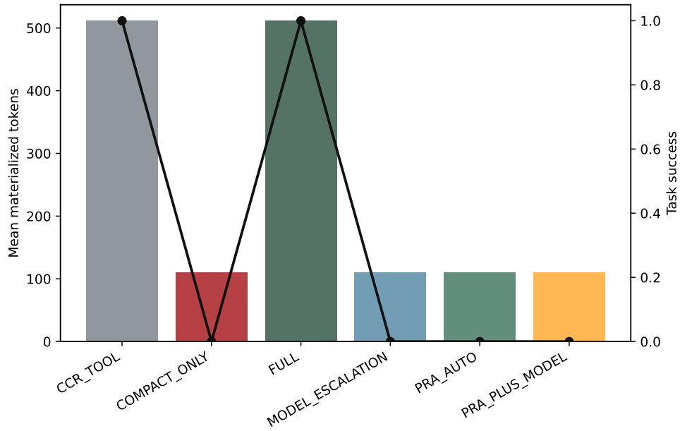
Figure 10: Cursor-class task success and materialized tokens. The repaired FULL and repeated-retrieval ceiling succeeds; the controller does not request the available cursor.
