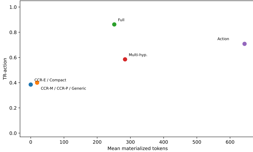
Figure 17: Mean materialized tokens versus latent TR-action. Policies at zero materialization can still exploit compact-view priors; policies farther right pay to expose exact backing evidence.
