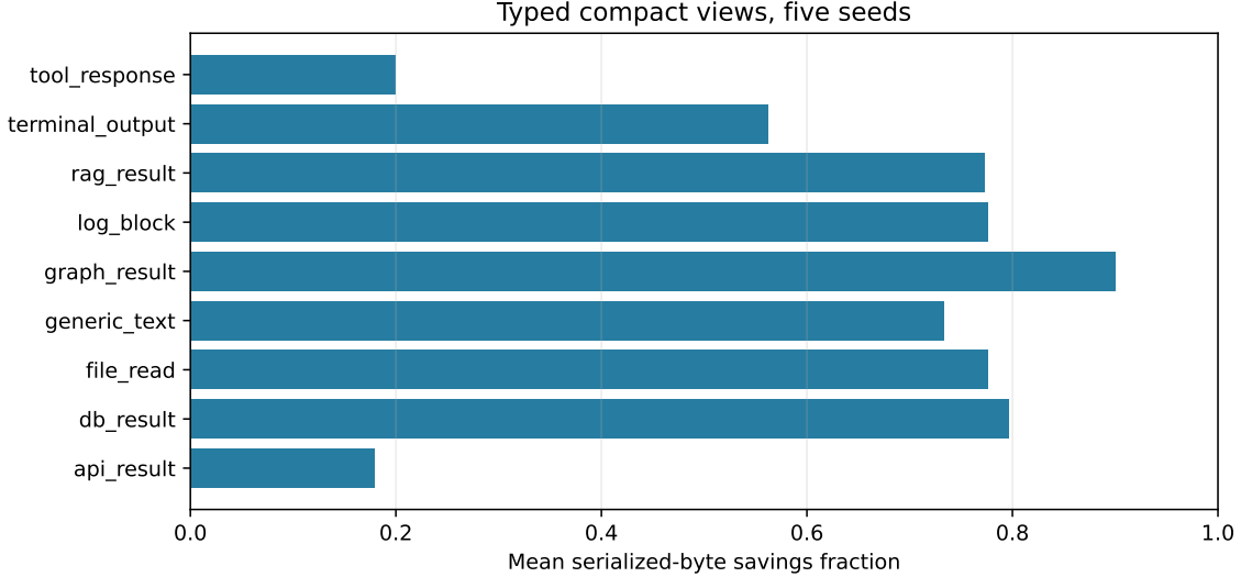
Figure 12: Mean serialized-byte savings by type across five seeds. Small structured tool/API fixtures have limited headroom; graph, database, log, and text-like results are substantially reduced.
