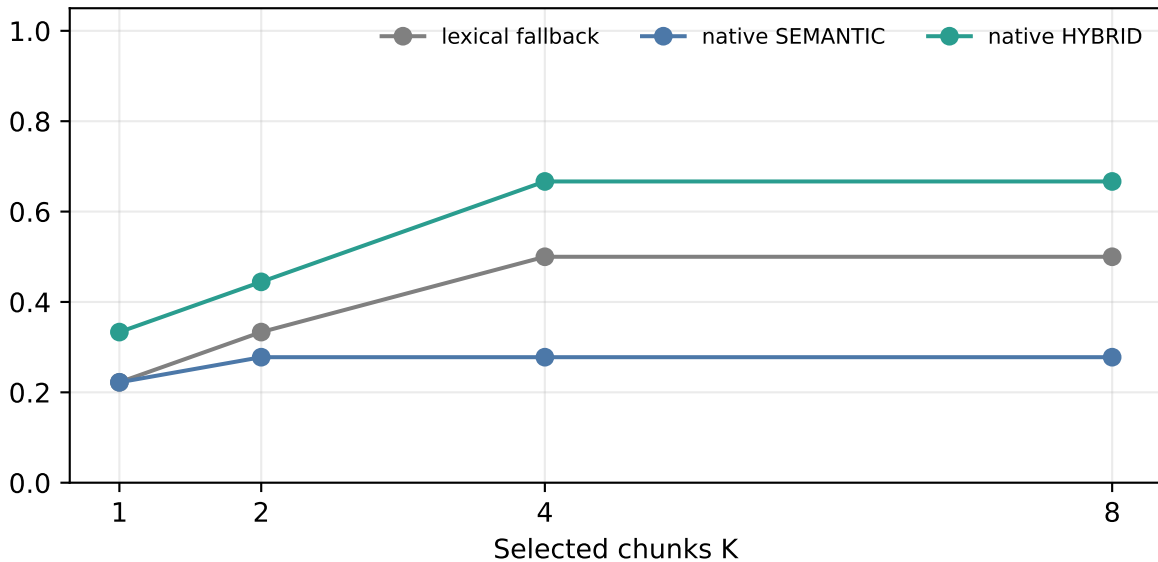
Backing evidence Recall@K
