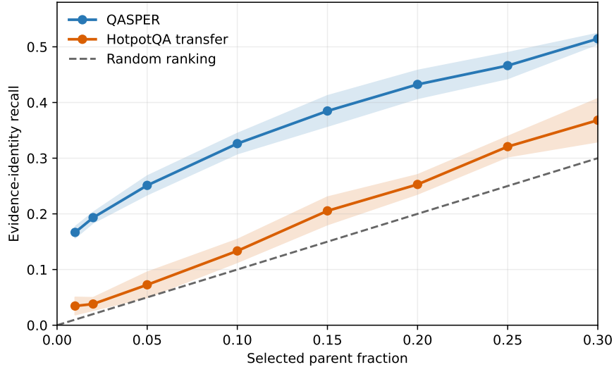
Figure 10: Gemma routing quality is sparse-budget and domain dependent. Five-seed evidence-identity recall is useful on QASPER, its training domain, and transfers more weakly to HotpotQA. Neither curve reaches 0.80 before exhaustive selection.
