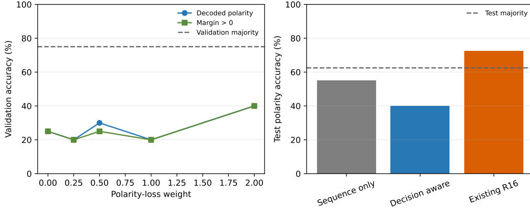
Figure 9: The bounded loss sweep improves validation polarity from 25% to 40% at \lambda = 2 but reverses on untouched test, where polarity falls from 55% to 40%. Dashed lines are the validation and test majority baselines. Explicit decision weighting is therefore insufficient in this small cohort.
