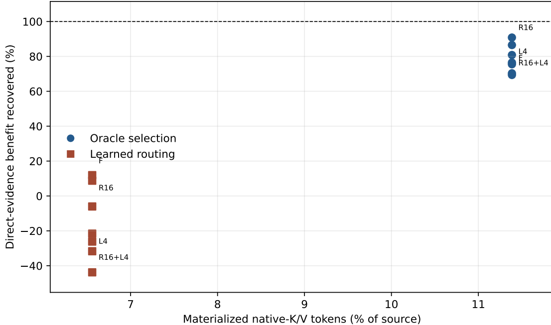
Figure 6: HotpotQA direct-evidence recovery versus physical native-K/V materialization. F, R16, L4, and R16+L4 label the frozen, residual-16, LoRA-4, and combined controls; unlabeled points are the remaining registered widths/ranks. All methods share a fixed memory fraction within a selection mode. Oracle residual 16 raises the ceiling, while every learned adaptation lowers the routed frontier relative to frozen PRA.
