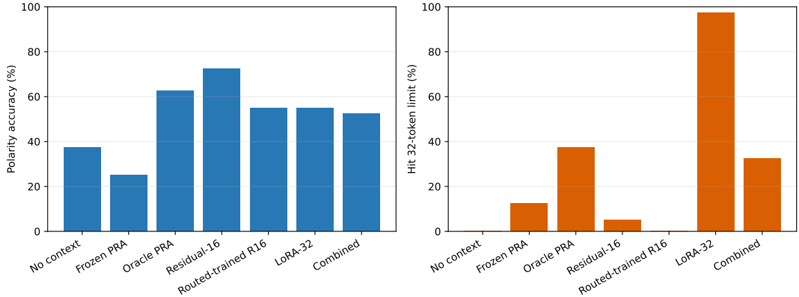
Figure 8: QASPER polarity accuracy and 32-token length termination. The residual adapter improves the evidence-conditioned decision while retaining natural completion. Rank-32 LoRA has a positive teacher-forced polarity margin but reaches the generation cap in 97.5% of trials; probability improvement alone therefore does not establish decoded utility.
