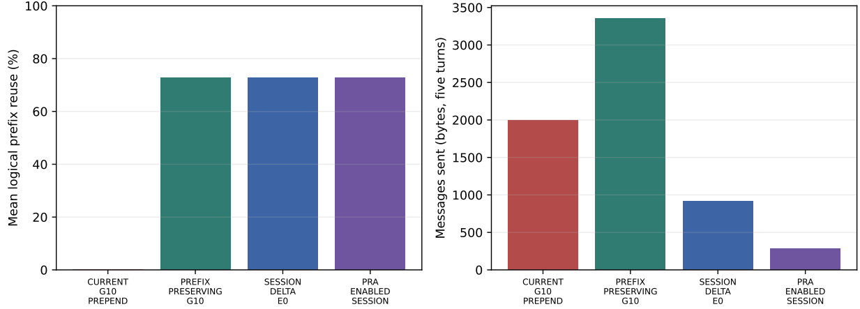
Figure 11: Five-turn deterministic gateway profile. The left panel reports logical reuse of the exact prior serialized message prefix after turn one; the right reports message bytes sent. Resource bytes are reported separately in Table 22.
