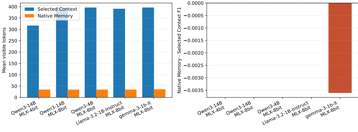
Figure 31: Observed visible-context accounting and Native-Memory-minus-Selected-Context token-F1 change by exact precision encoding. The plot deliberately excludes planned rows; absence is not rendered as zero.
