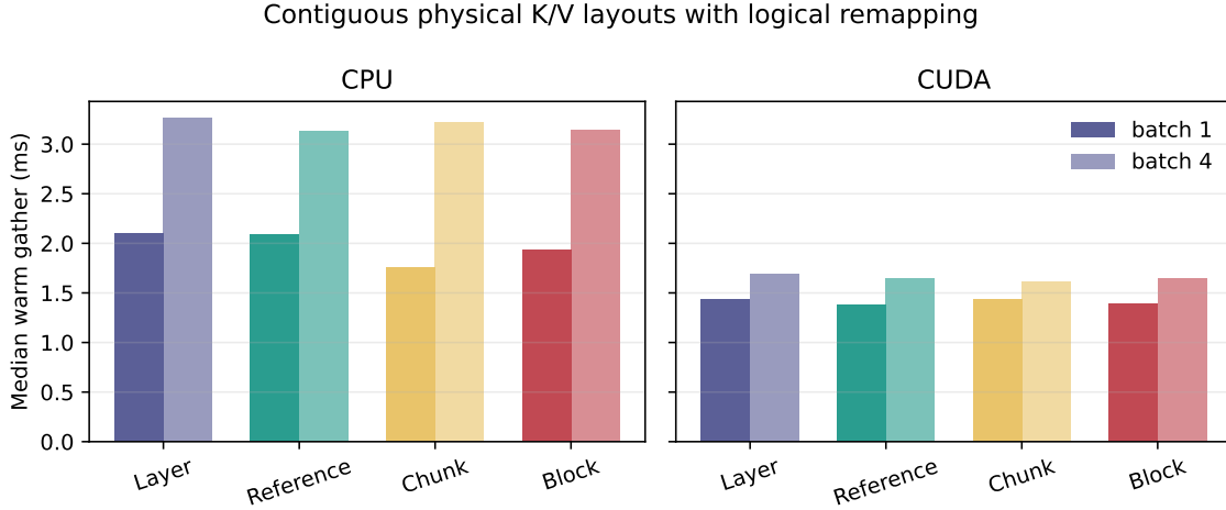
Figure 17: Warm materialization from four physically distinct contiguous stores. Every layout restores the same logical per-layer K/V before attention.
