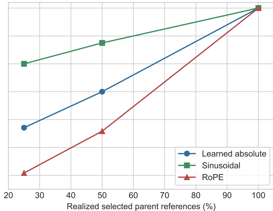
QASPER-derived
