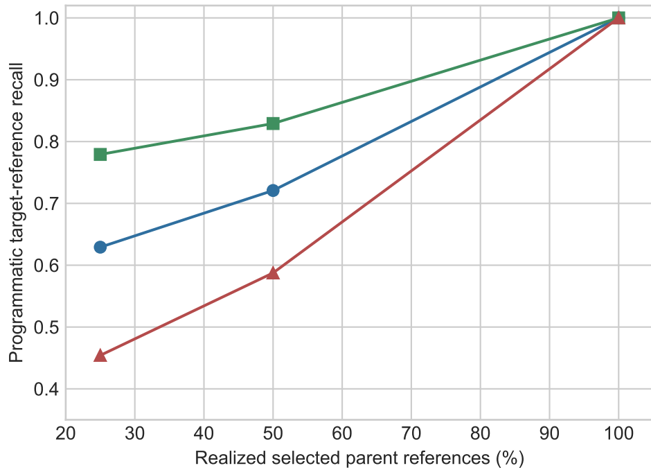
HotpotQA-derived
