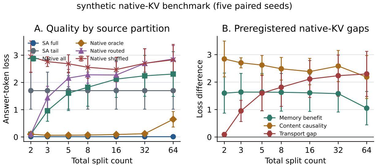
Figure 3: Five-seed fixed-source synthetic native-KV result. Full-context SelfAttention solves the dependency while the local tail is at chance. Oracle memory preserves the required content through 32 splits and sharply separates from shuffled content. Native-all and unsupervised routed conditions degrade as the same source is fragmented, distinguishing successful sparse transport from unresolved cache-composition and selection behavior. Error bars are population standard deviations.
