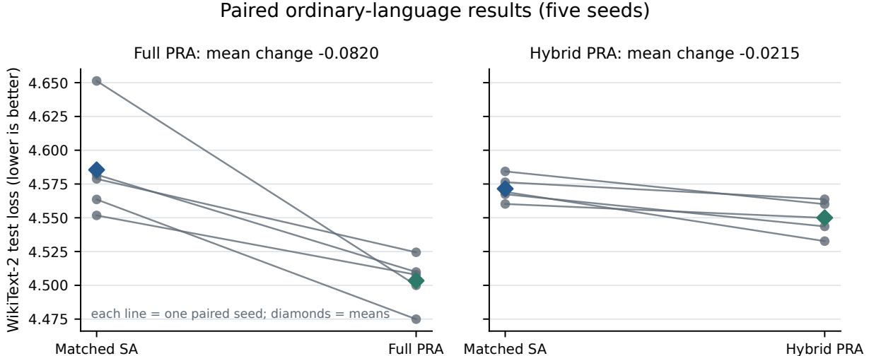
Figure 4: Paired ordinary-language losses for the historical cross-attention-capable backbones. Each line connects one seed to its nearly parameter-matched SelfAttention control; diamonds mark five-seed means. External memory is absent in these runs. The directional result is encouraging but underpowered ( p = 0.0625 ), and it is not a native-KV quality measurement.
