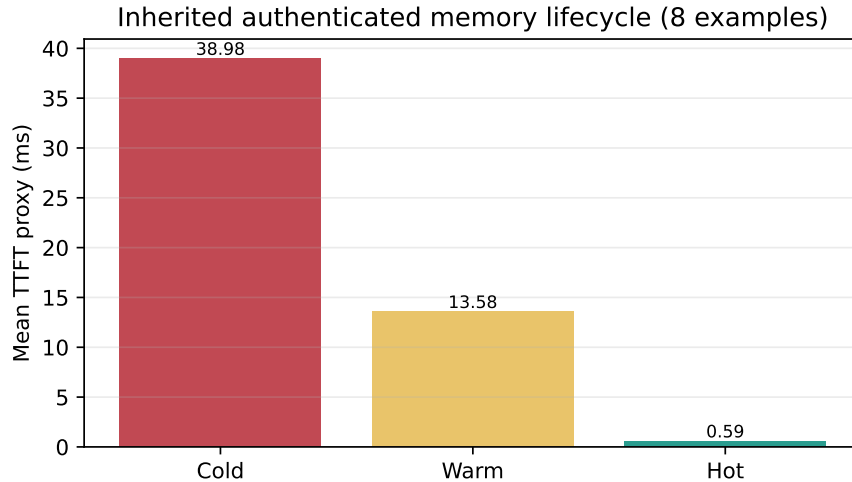
Figure 14: Inherited Paper 4 lifecycle proxy over eight examples. Cold includes fetch and native encoding; warm reuses native encoding; hot reuses selected K/V.
