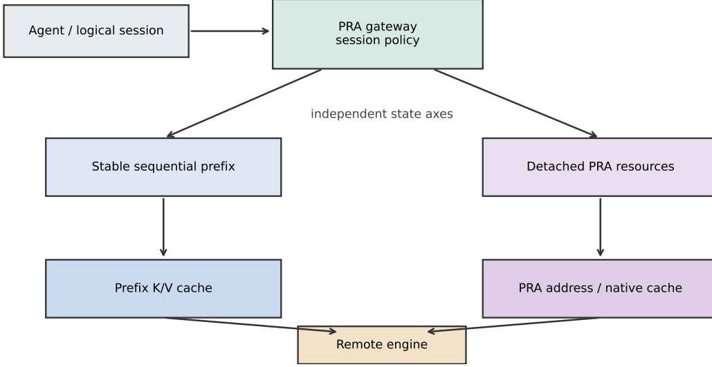
Figure 5: The session-aware gateway maintains two independent state axes. Sequential prompt K/V follows the engine’s ordinary prefix-cache policy; detached PRA resources follow the PRA lifecycle and may be text-materialized at E0 or retained natively at E1+.
