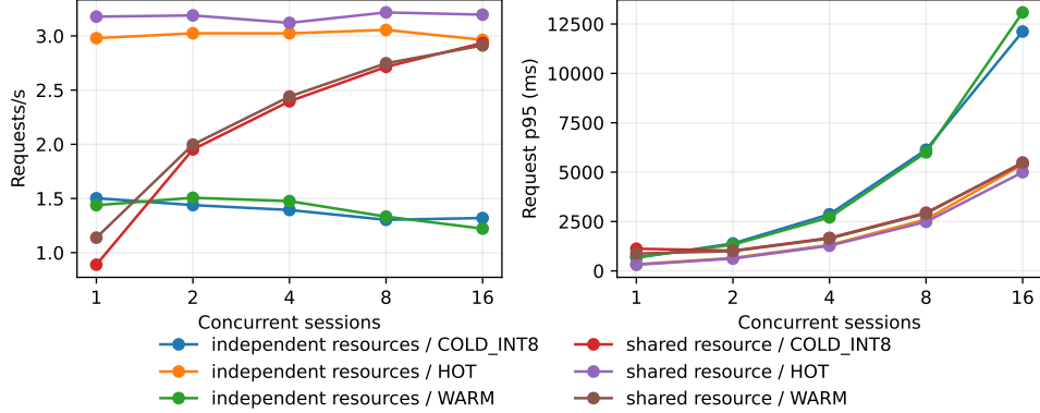
Figure 20: Shared and independent MLX resources through 16 concurrent sessions. The finite waves include promotion and serialized model queueing.
