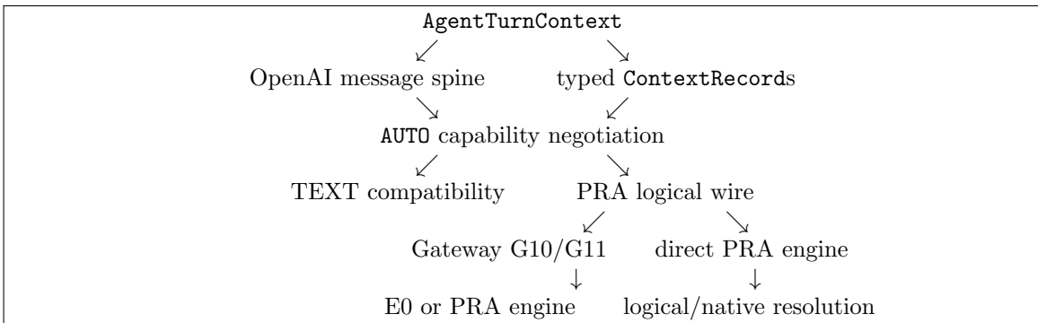
Figure 4: The agent preserves the pretrained conversational spine separately from detached typed context. Compatibility loss occurs only at an explicit TEXT or G10 downgrade; native K/V remains engine-side.
