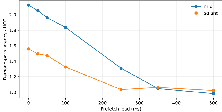
Figure 19: Scheduler-owned WARM promotion can hide request-path stall when useful lead is available. The dashed line is HOT latency.
