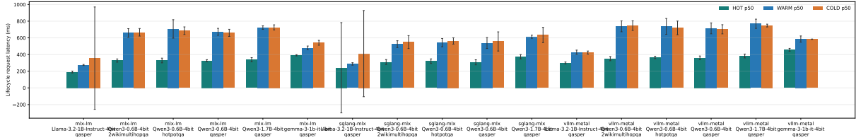
Figure 26: HOT, WARM, and COLD request p50 with p95–p50 upper whiskers. WARM recovery is reliable, but synchronous promotion remains visibly expensive.
