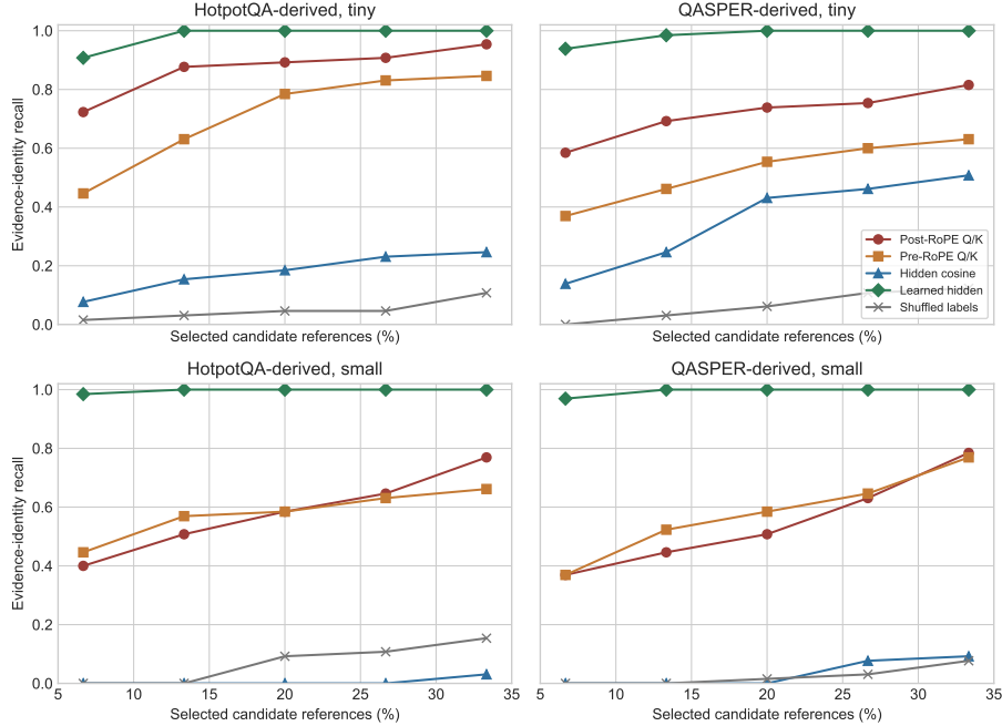
Figure 8: The learned 32-D hidden-state metric dominates raw hidden cosine and the shuffled-label control throughout the sparse range. Post-RoPE and pre-RoPE Q/K remain useful controls but do not define the best evidence-ranking geometry. Curves average five seeds.
