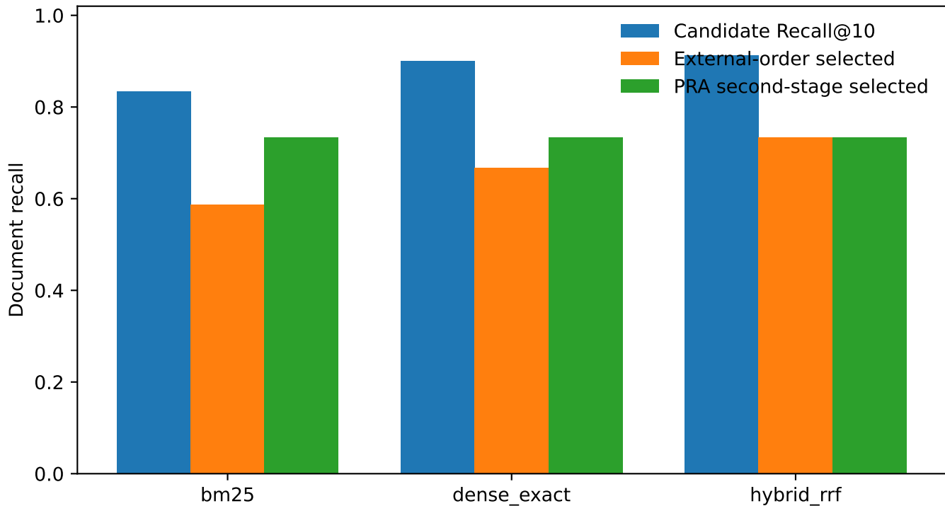
Synthetic retrieval and frozen-selection mechanism smoke
