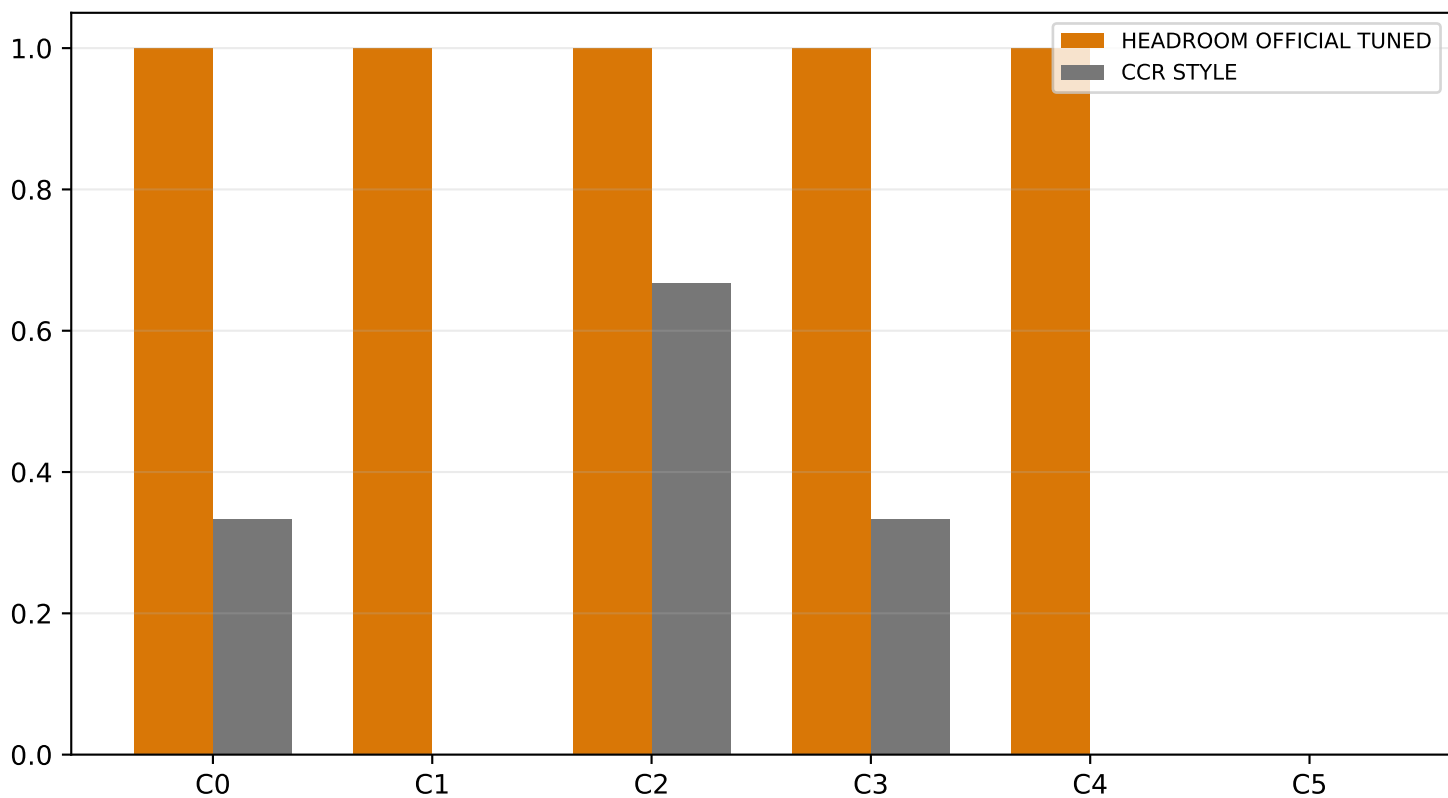
Trigger/action accuracy
