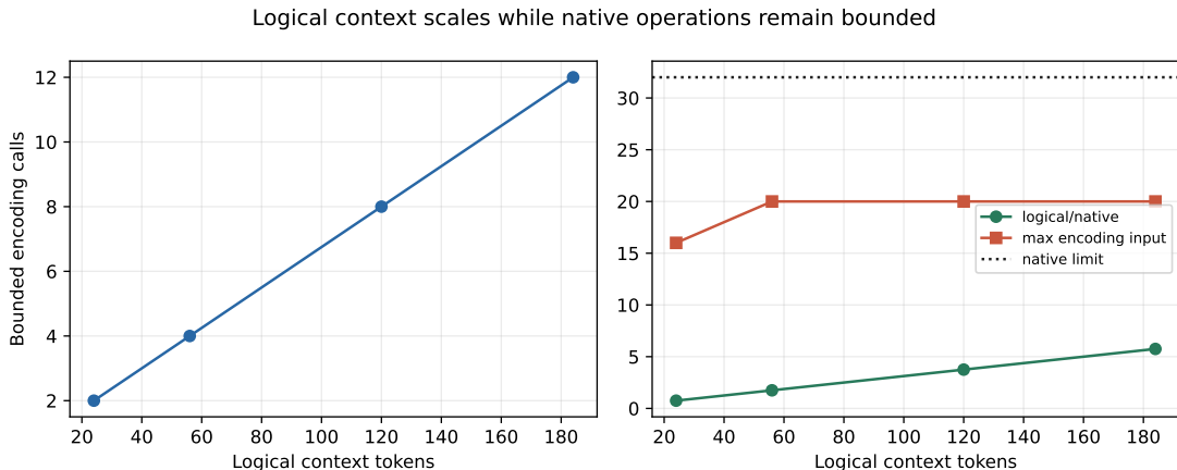
Figure 22: Model-scaled context safety. Logical head length and encoding-call count grow, while each overlap-aware base-model encoding remains below the 32-token hard limit.
