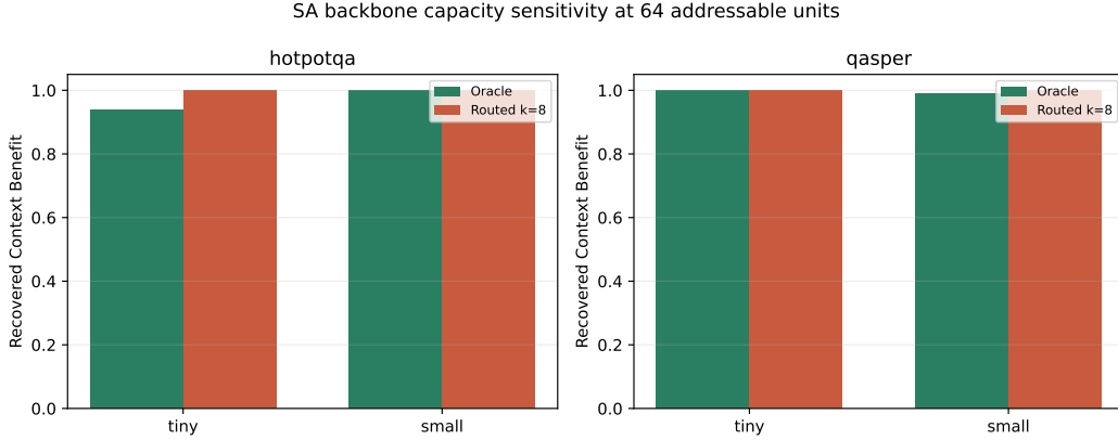
Figure 16: Backbone capacity at 64 units. The small tier improves annotated-oracle robustness and maintains routed quality, but also increases model and K/V width.
