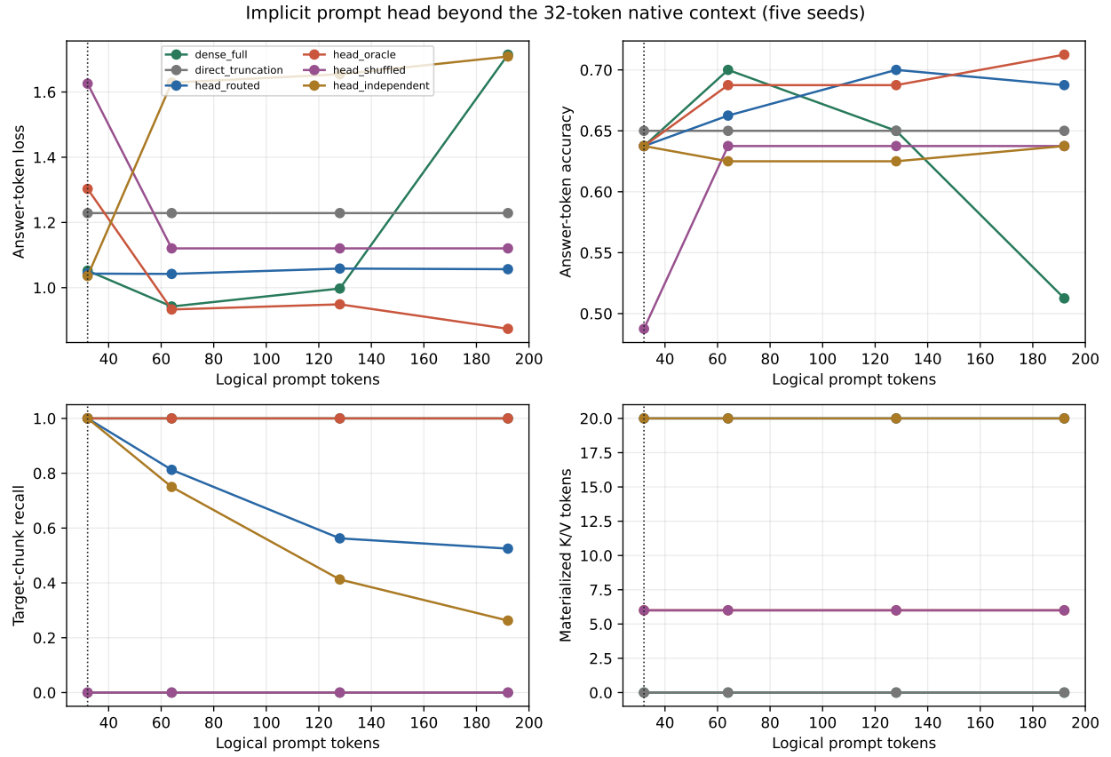
Figure 23: Quality, recall, and active memory as the implicit head grows beyond the native limit. Dense execution is shown only because this tiny source model supports 192 tokens.
