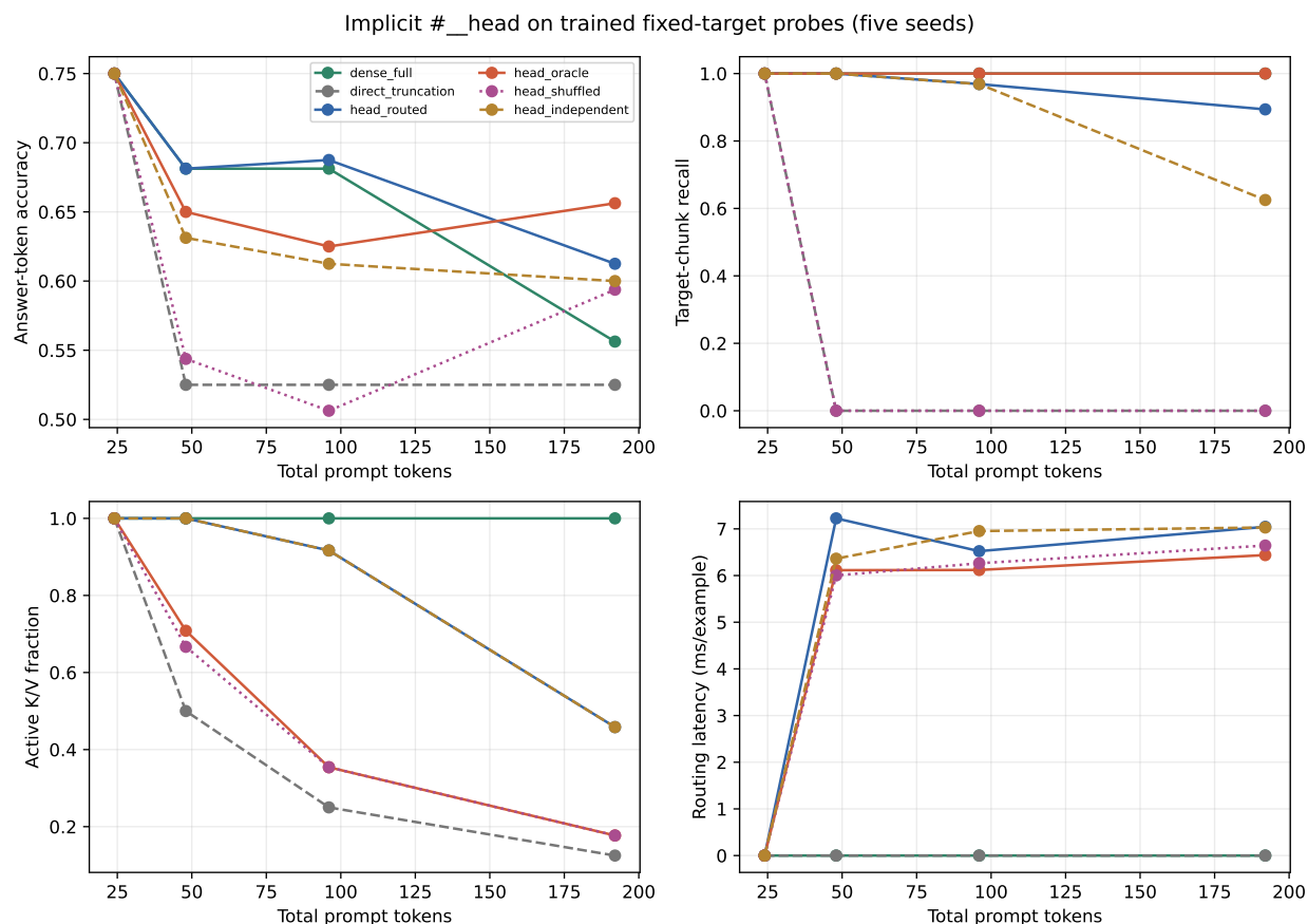
Figure 20: Implicit-head quality through eight times the direct budget. Historical slicing, truncation, wrong memory, and independent chunk encoding isolate access, content causality, and contextual fragmentation.
