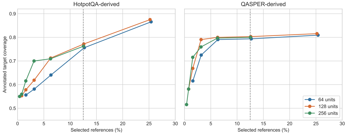
Figure 15: Measured coverage curves for the final small-tier native-slice router. The vertical line marks 12.5%. Only stored k \in \{1, 2, 4, 8, 16, 32\} points inside the 0–30% region are connected.
