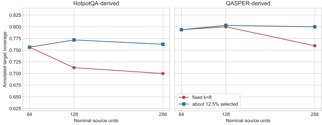
Figure 14: Fixed k = 8 becomes progressively more selective as the candidate set grows. Holding the selected-reference fraction near 12.5% instead keeps annotated coverage nearly constant from 64 through 256 units.
