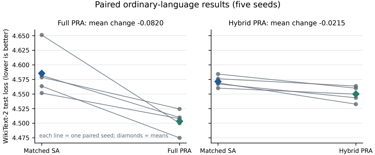
Figure 27: Paired ordinary-language losses for the historical cross-attention-capable backbones. Each line connects one seed to its nearly parameter-matched SelfAttention control; diamonds mark five-seed means. External memory is absent in these runs. The directional result is encouraging but underpowered ( p = 0.0625 ), and it is not a native-KV quality measurement.
