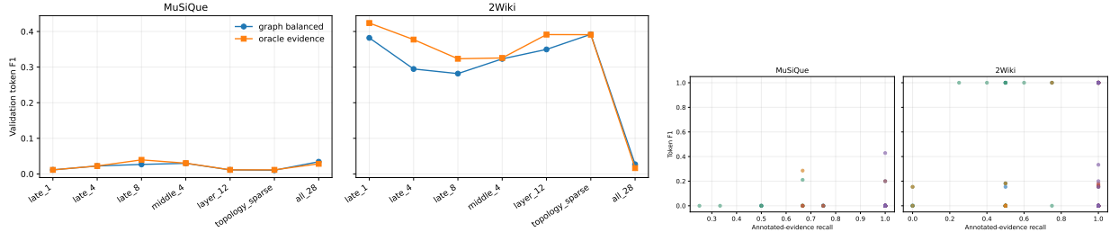
Figure 14: Left: fixed evidence under different consumption bands. All-layer injection collapses 2Wiki output. Right: annotated-evidence recall is not sufficient for answer quality.
