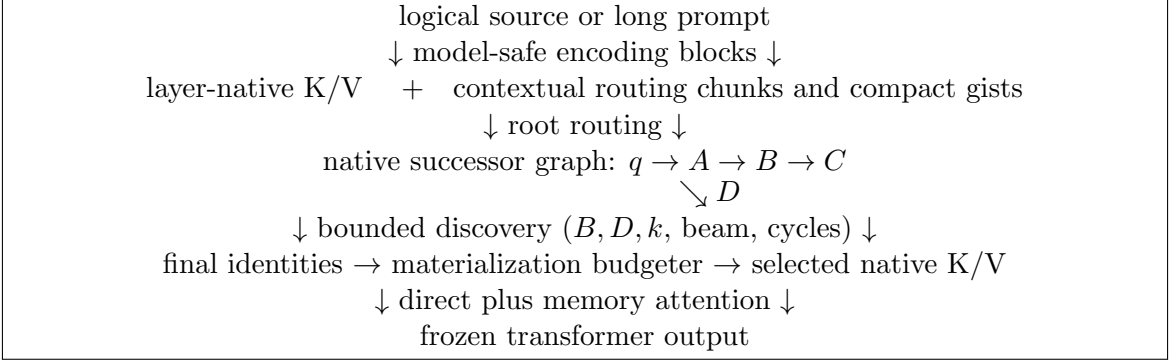
Figure 8: Final computational decomposition. Iterative PRA increases discovery depth without transformer reruns. Compact gists and native edges define routing state; selected layer-native K/V is the attention payload.
