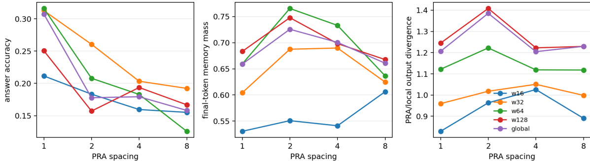
Figure 4: PRA spacing over in-domain depths 1–4. More frequent interventions improve discovery at higher K/V cost. Memory mass and output divergence confirm active, sometimes disruptive native-K/V consumption rather than a silent routing path.
