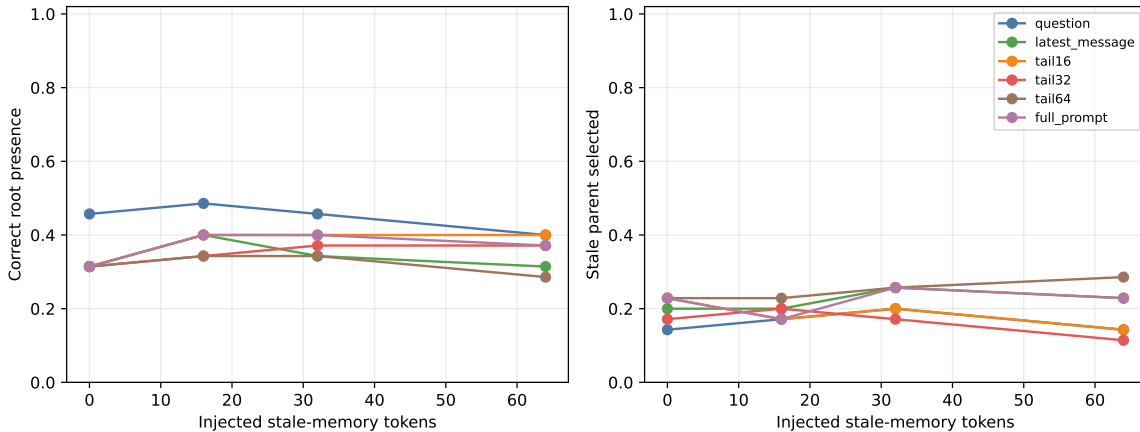
Figure 26: Held-out Hotpot response to injected stale-memory text. Left: current root entry. Right: selection of the explicitly non-oracle stale parent. The validation-frozen latest-message boundary is bounded and cheaper, but stale-context resistance remains mixed on this sample.
