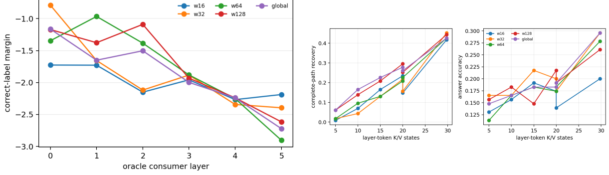
Figure 7: Left: the matched oracle memory-use profile is strongest in early consumer layers. Right: more layer-token K/V states generally improve path recovery, while answer accuracy is non-monotonic. Every-layer PRA is retained as a diagnostic frontier, not a proposed deployment policy.
