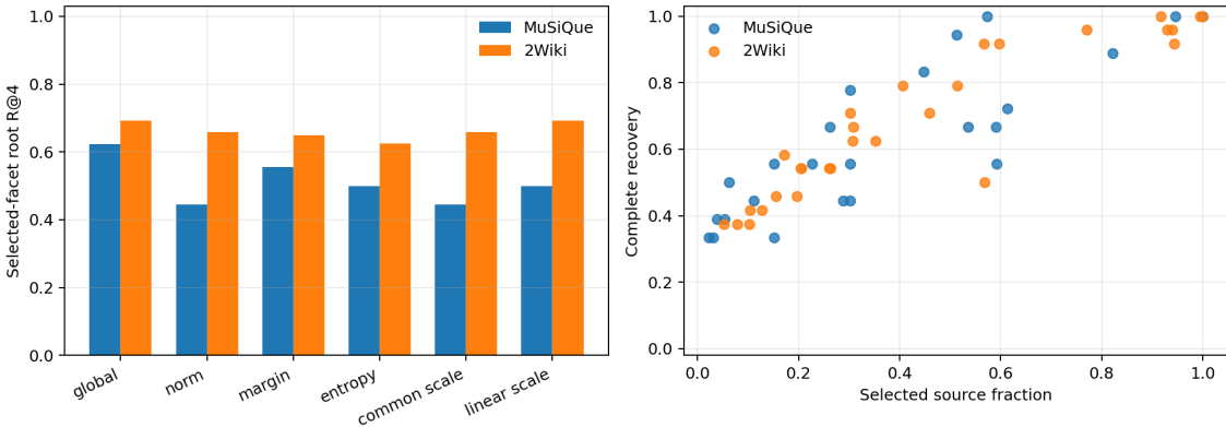
Figure 12: Left: executable facet selectors remain below the oracle root-view ceiling. Right: high complete recovery requires broad conceptual source activation.
