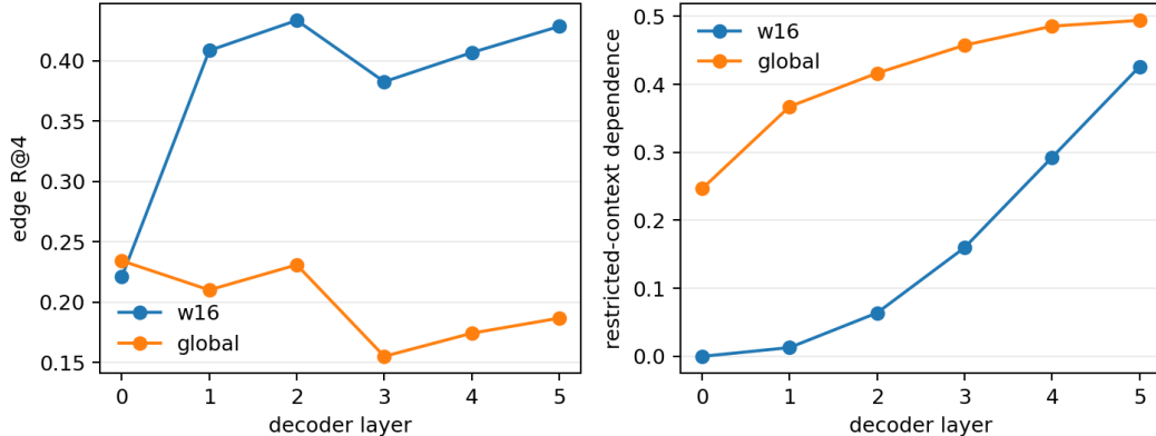
Figure 2: Layerwise edge R@4 and dependence on context outside a 16-token tail. Local states become contextual through depth without collapsing to the global model’s shortcut-rich topology.
