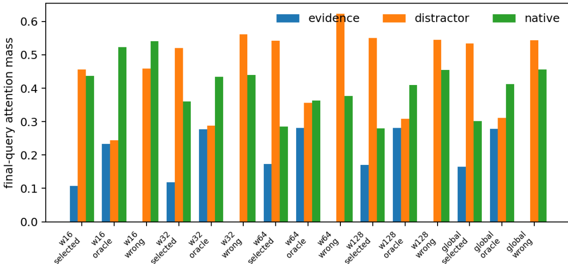
Figure 5: Exact final-query shared-softmax decomposition for iterative selected, oracle, and wrong memory. Selected memory is distractor dominated. Oracle forcing approximately doubles evidence mass while preserving a matched physical payload.
