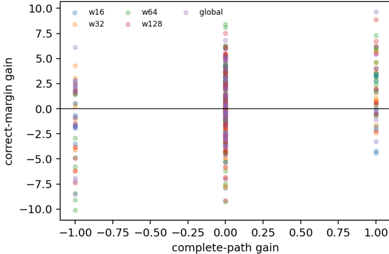
Figure 6: Paired complete-path and correct-margin changes for iterative versus one-shot PRA. Better paths tend to move the frozen decision in the correct direction, but most rows do not improve the path and some lose it. Points are diagnostic model-example units, not independent model seeds.
