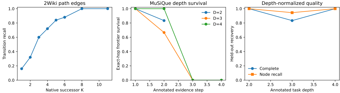
Figure 9: Natural graph diagnostics. 2Wiki exposes transition/path fidelity; MuSiQue separates annotated task depth from minimum native recovery depth.
