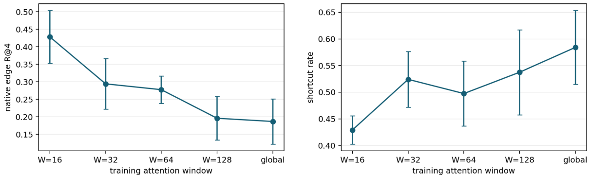
Figure 1: Final-layer native topology versus the trained attention window. Error bars are five-seed 95% Student- t intervals. Narrow local attention preserves more evidence edges and forms fewer non-adjacent shortcuts.
