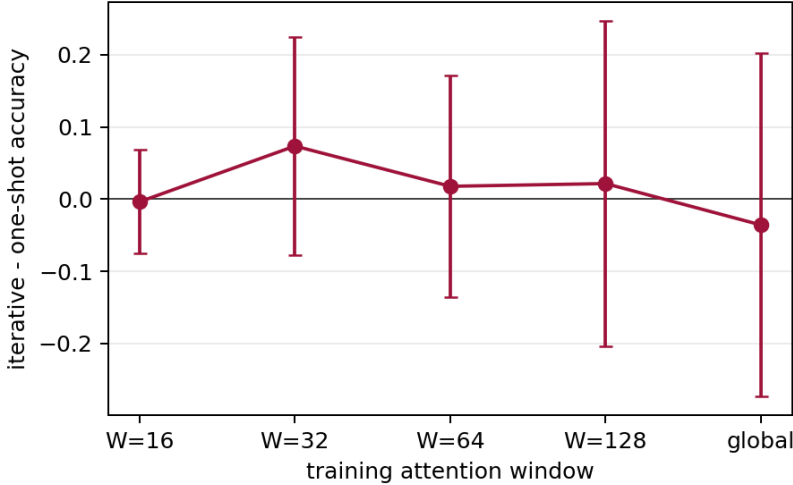
Figure 3: Paired depth-macro answer-accuracy gain of matched iterative PRA over one-shot PRA. No window resolves a nonzero effect with five seeds.
