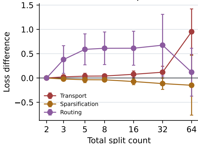
D. Error decomposition
