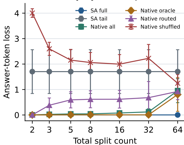
A. Quality by source partition
