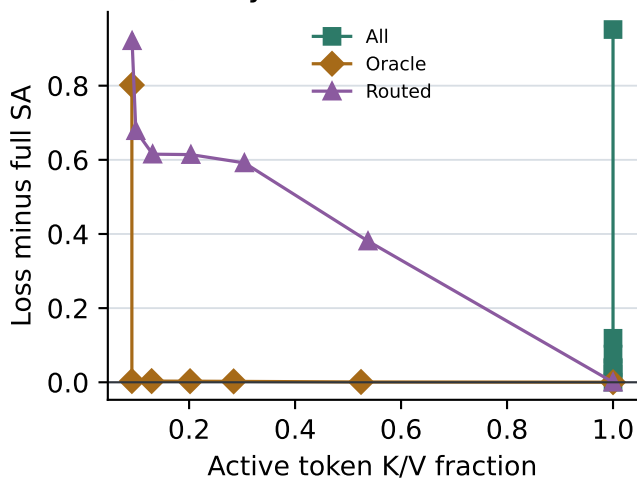
C. Quality-active-context frontier
