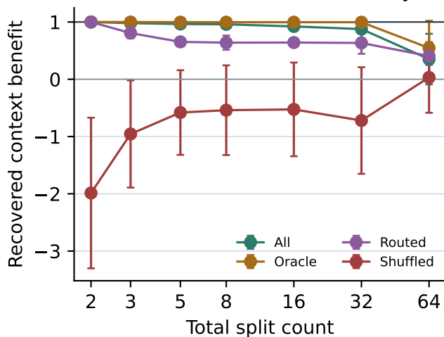
B. Context benefit recovery
