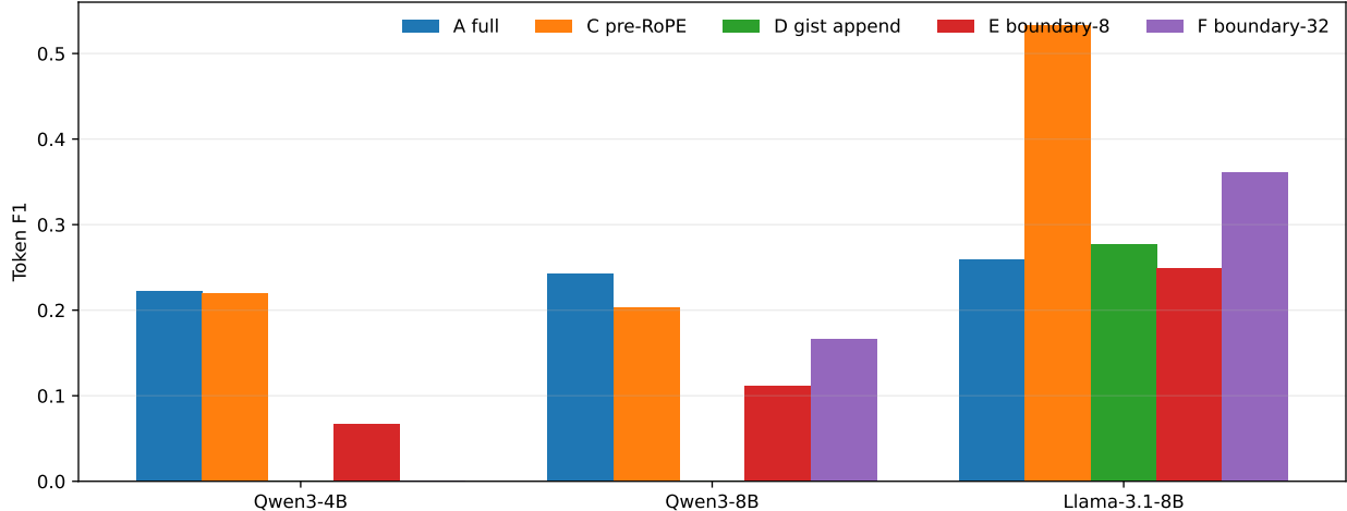
Figure 16: Token F1 in the reduced cross-model mechanism pilots. The Llama cohort shows less severe degradation, but no parameter-free composition arm improves on independent pre-RoPE K/V.
