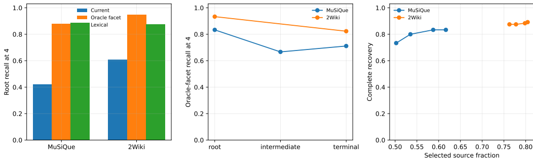
Figure 26: All-offset query audit. Left: current, oracle-facet, and lexical root R@4. Center: semantic visibility by evidence role. Right: the bounded executable union spends more source without realizing the oracle ceiling.
