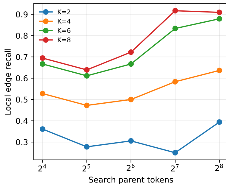
MuSiQue: frozen native graph granularity
