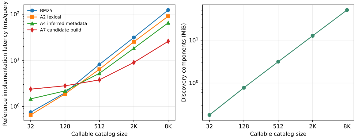
Figure 24: Reference implementation latency and measured discovery-component memory. Both axes are logarithmic; query encoding is batched and reported separately in the machine-readable cost rows.
