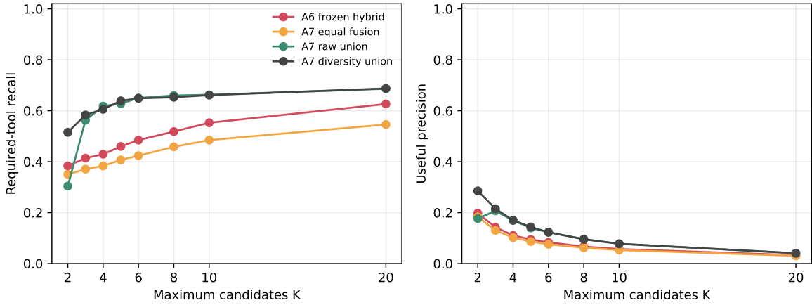
Figure 23: The 8,192-tool matched-budget frontier. Candidate-set recall and useful precision must be read together.
