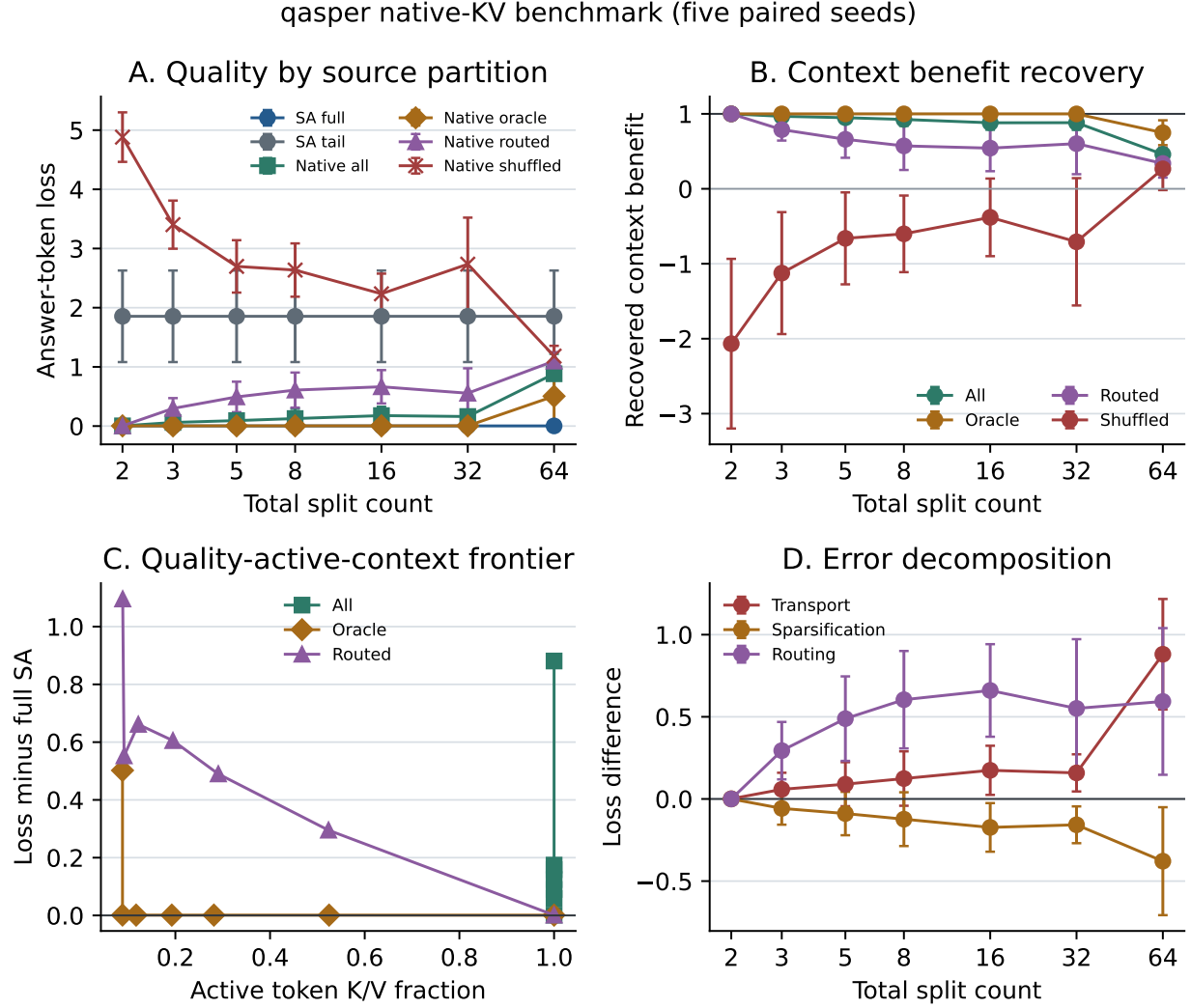
Figure 7: QASPER-derived quality and error decomposition over five paired seeds. Oracle native K/V preserves dense-context quality through split 32, while all-memory composition and routed selection accumulate distinct errors.
