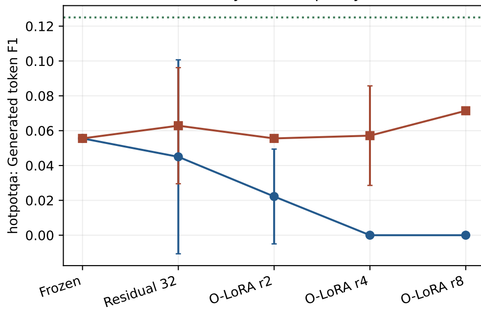
Greedy answer quality
