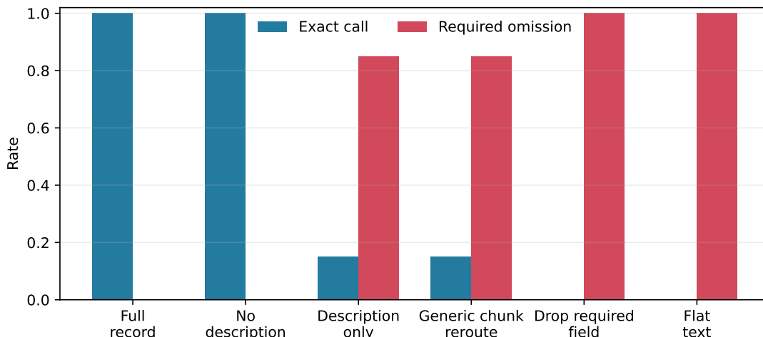
Figure 22: E5–E6 exact calls and required-argument omissions. The generic router selects one internal schema segment; all partial-schema conditions are experimental controls, not runtime fallback policies.
