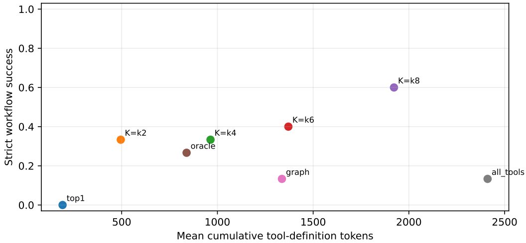
Figure 21: E4 strict workflow success against cumulative visible schema tokens. The frozen model, host authorization, and pure handlers are unchanged across candidate policies.
