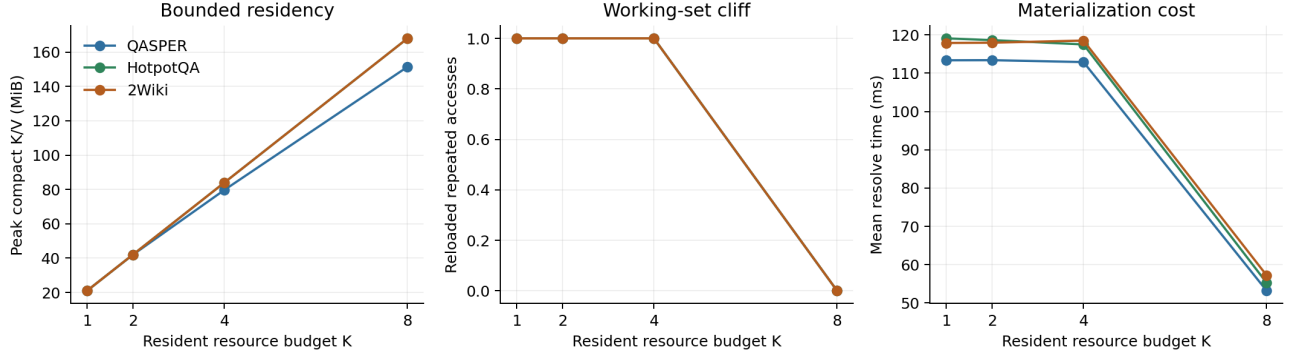
Figure 6: Five-seed compact-K/V pressure over QASPER, HotpotQA, and 2Wiki. Each seed visits eight resources twice and then revisits the first. The budget K = 8 is the first condition that fits the working set.
