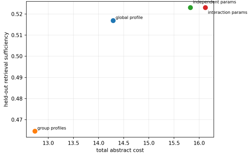
Figure 19: Target-architecture quality/cost frontier. Parameter heads improve over grouped modes, but none approaches the robust profile selector; low-cost group routing is under-allocation.
