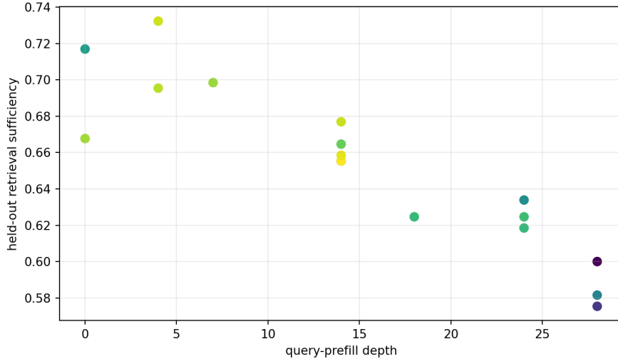
Figure 17: Held-out profile-router quality over query-prefill depth. Color encodes total abstract cost. Greater depth does not produce a monotonic quality gain.
