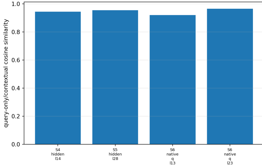
Figure 18: Cosine similarity between pooled query-only and 256-token source-contextualized question states. Contextual processing is expensive, while the selected representations remain close.
